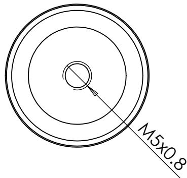
Small Ribbed Cupboard Knob: Ø 25 mm, Projection 29 mm (Base Ø 17 mm)
