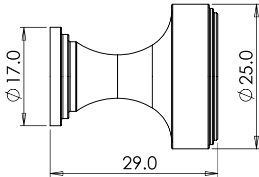
Small Ribbed Cupboard Knob: Ø 25 mm, Projection 29 mm (Base Ø 17 mm)
