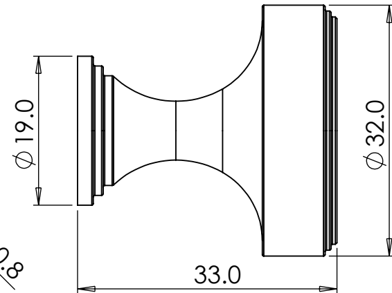
Large Ribbed Cupboard Knob: Ø 32 mm, Projection 33 mm (Base Ø 19 mm)
