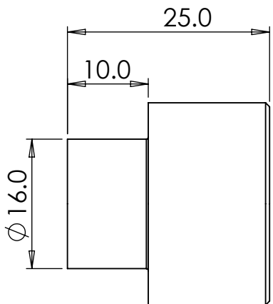
Small Stepped Knob - Ø 25 mm
