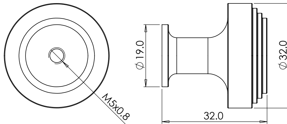
Large Sweep Stepped Cupboard Knob Ø 32 mm, Projection 32 mm (Base Ø 19 mm)
