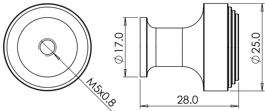
Small Sweep Stepped Cupboard Knob Ø 25 mm, Projection 28 mm (Base Ø 17 mm)
