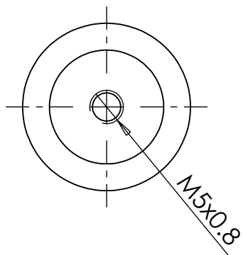
Small Ringed Cupboard Knob: Ø 25 mm, Projection 40 mm (Base Ø 17 mm)
