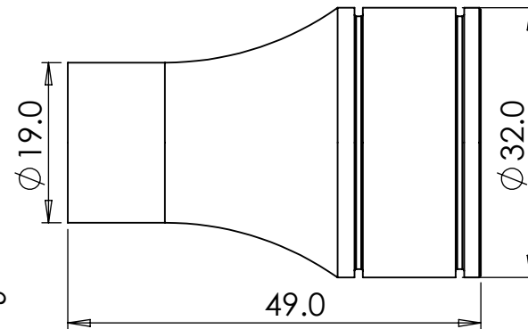
Large Ringed Cupboard Knob: Ø 32 mm, Projection 49 mm (Base Ø 19 mm)
