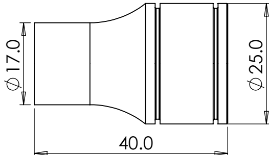
Small Ringed Cupboard Knob: Ø 25 mm, Projection 40 mm (Base Ø 17 mm)
