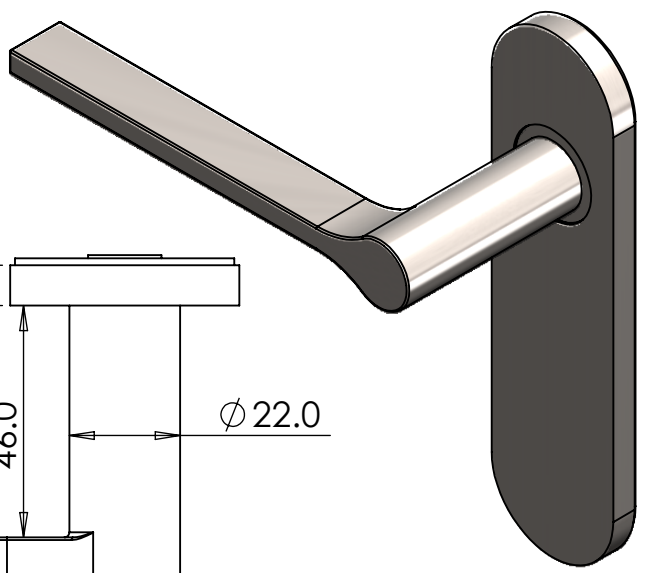
Isometric View Scale 1:2
