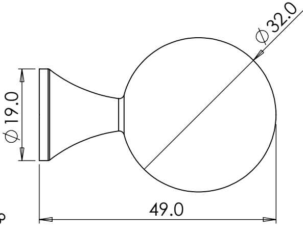
Large Sweep Knob
