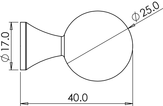
Small Sweep Knob
