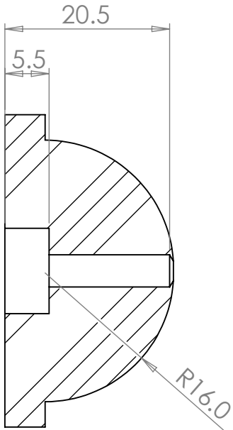
SECTION B-B
