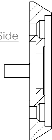
SECTION C-C
