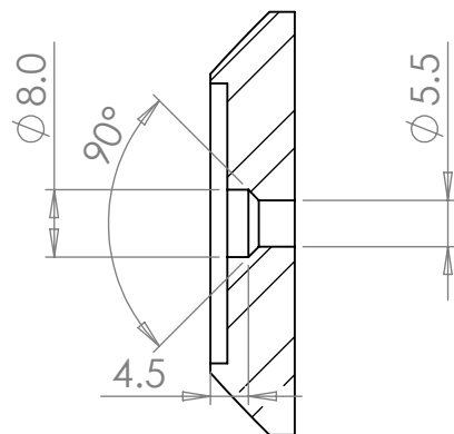
SECTION A-A 2 Positions
