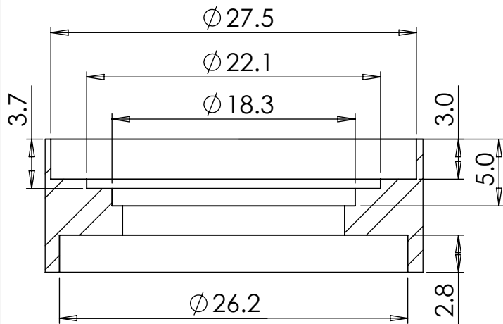
DETAIL B SCALE 2.5 : 1
