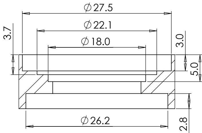
DETAIL D SCALE 2.5 : 1
