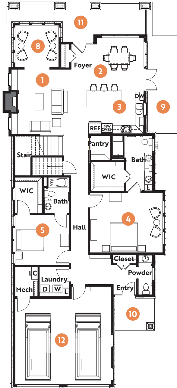
FIRST FLOOR
