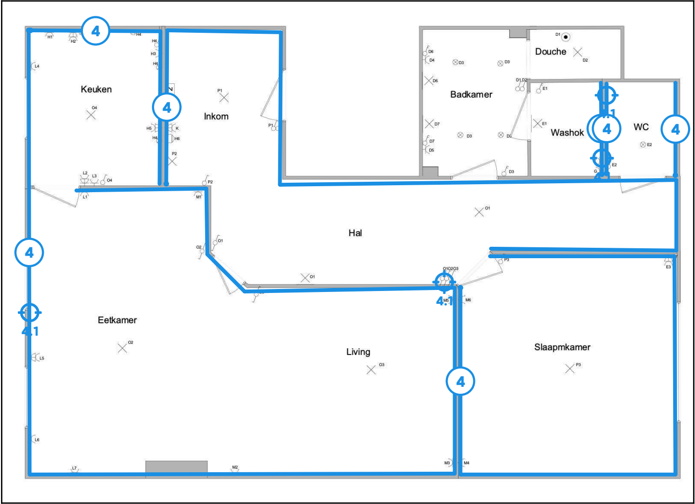
Legende van plan 1.4: Appartement +1 (wanden)
