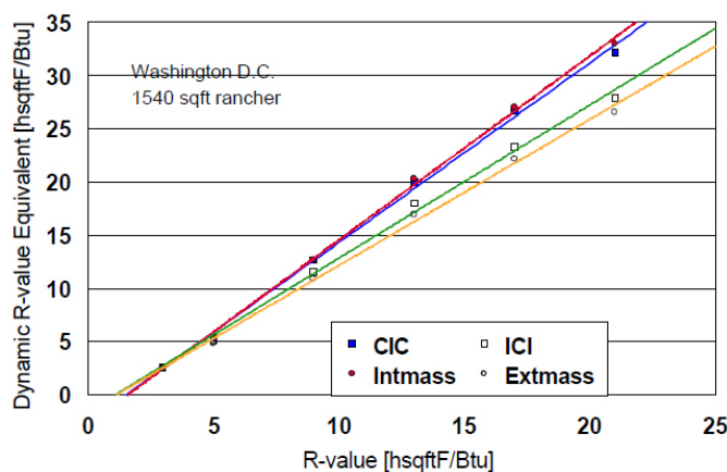
Fig.3. Dynamic R-value Equivaents for Washingtonn D.C. for 1540 ft 2 one-story rancher.
