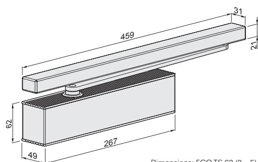
Dimensions: ECO TS-62 (2 – 5)
