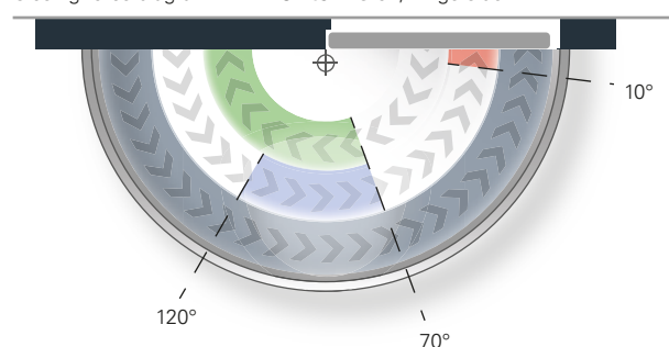
Closing force diagram ECO Newton TS-62, hinge side
