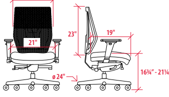
GM33 Mesh Back w/ Standard Seat
