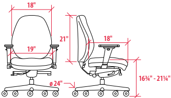
GFU22 Mid Back w/ Medium Seat
