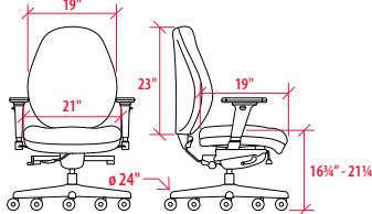
GFU33 Standard Back w/ Standard Seat
