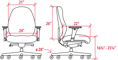
GFU44 Highest Back w/ Extra Large Seat
