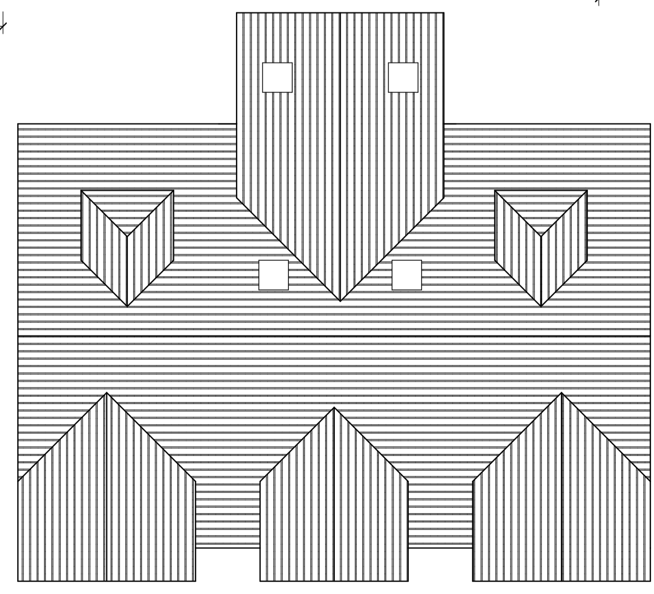
Roof Plan
