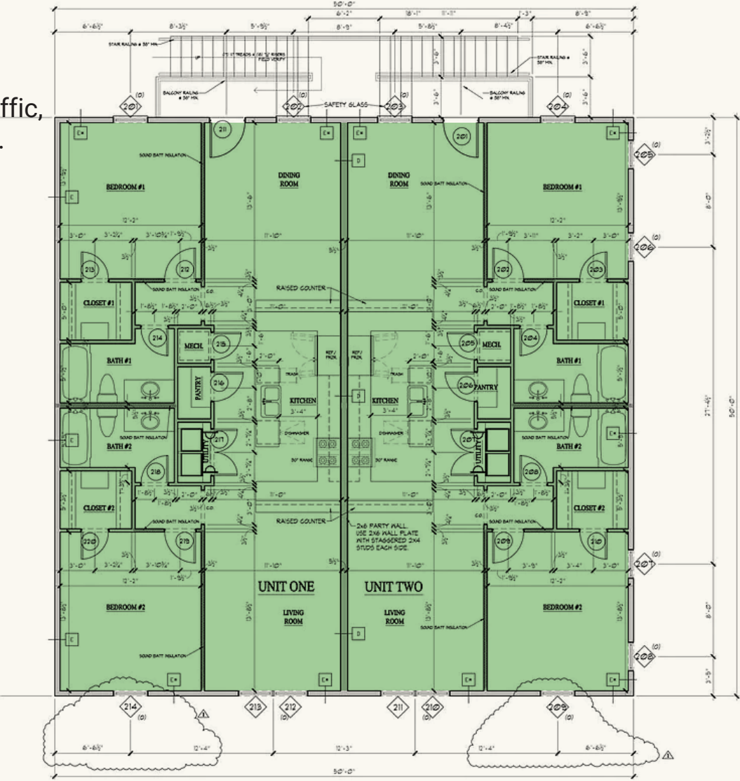
2 SECOND FLOOR PLAN SCALE: 1/4" = 1'-0"
