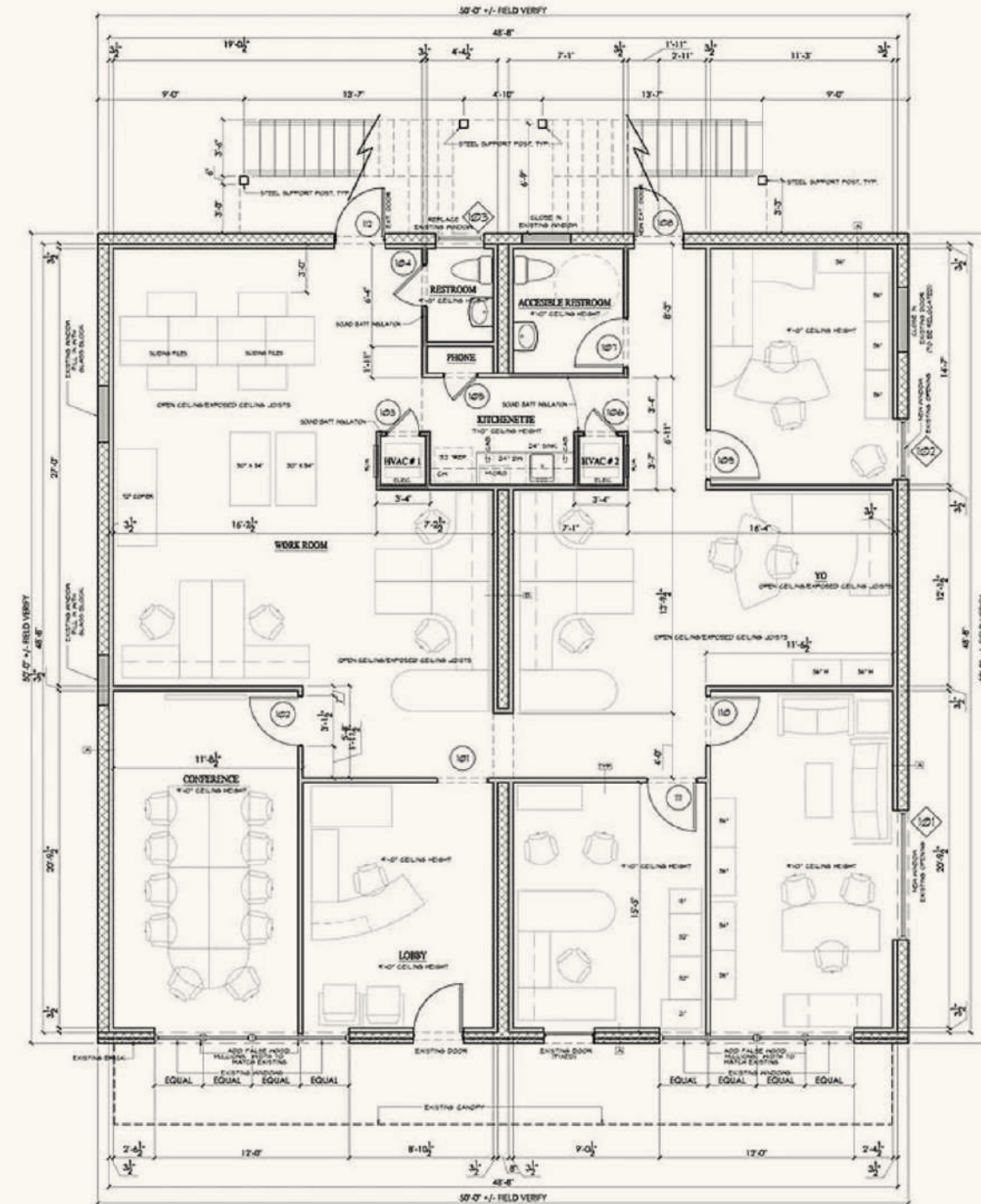
1 FIRST FLOOR PLAN SCALE: 1/4" = 1'-0"
