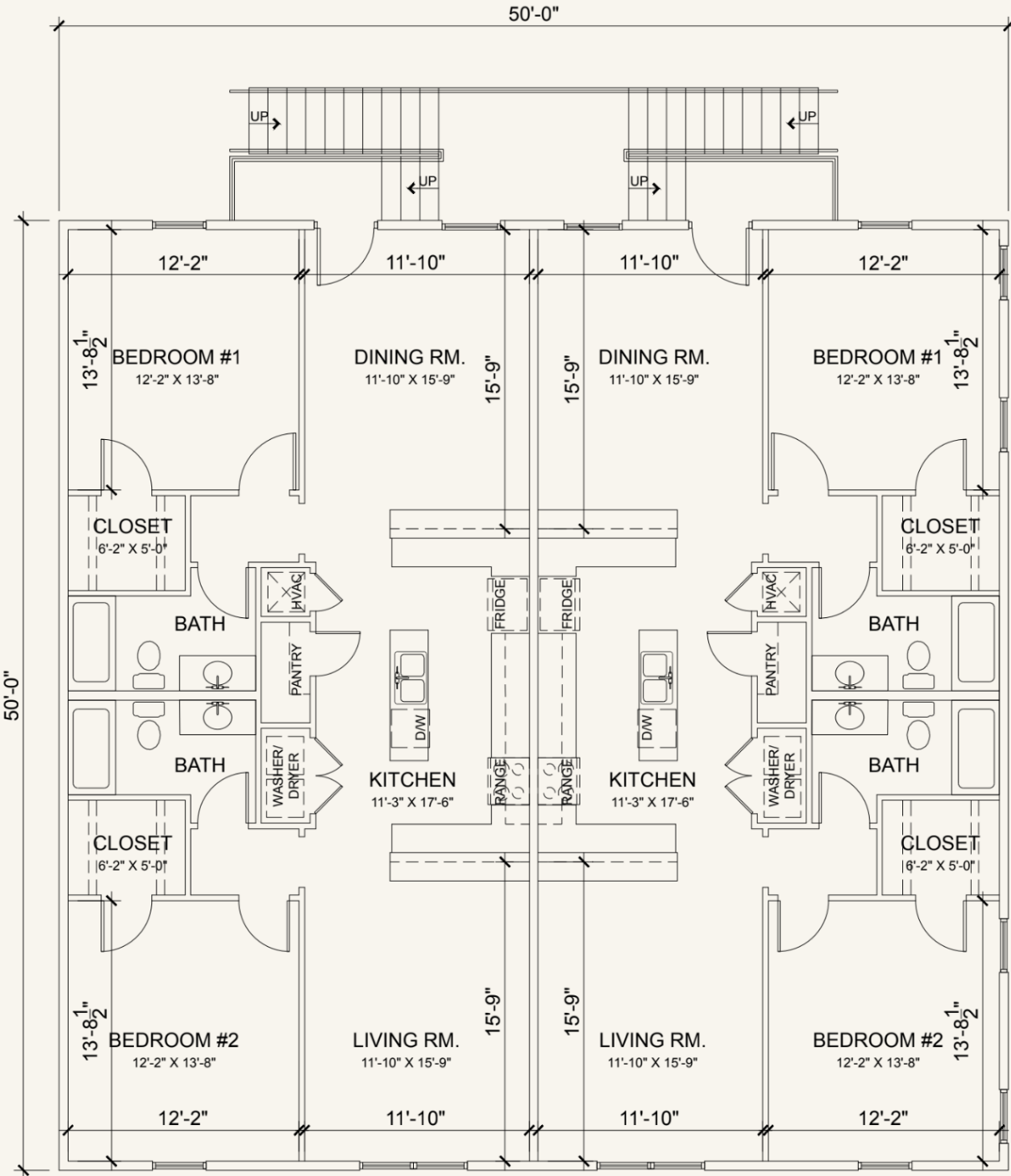
LEVEL 2 - RESIDENTIAL
