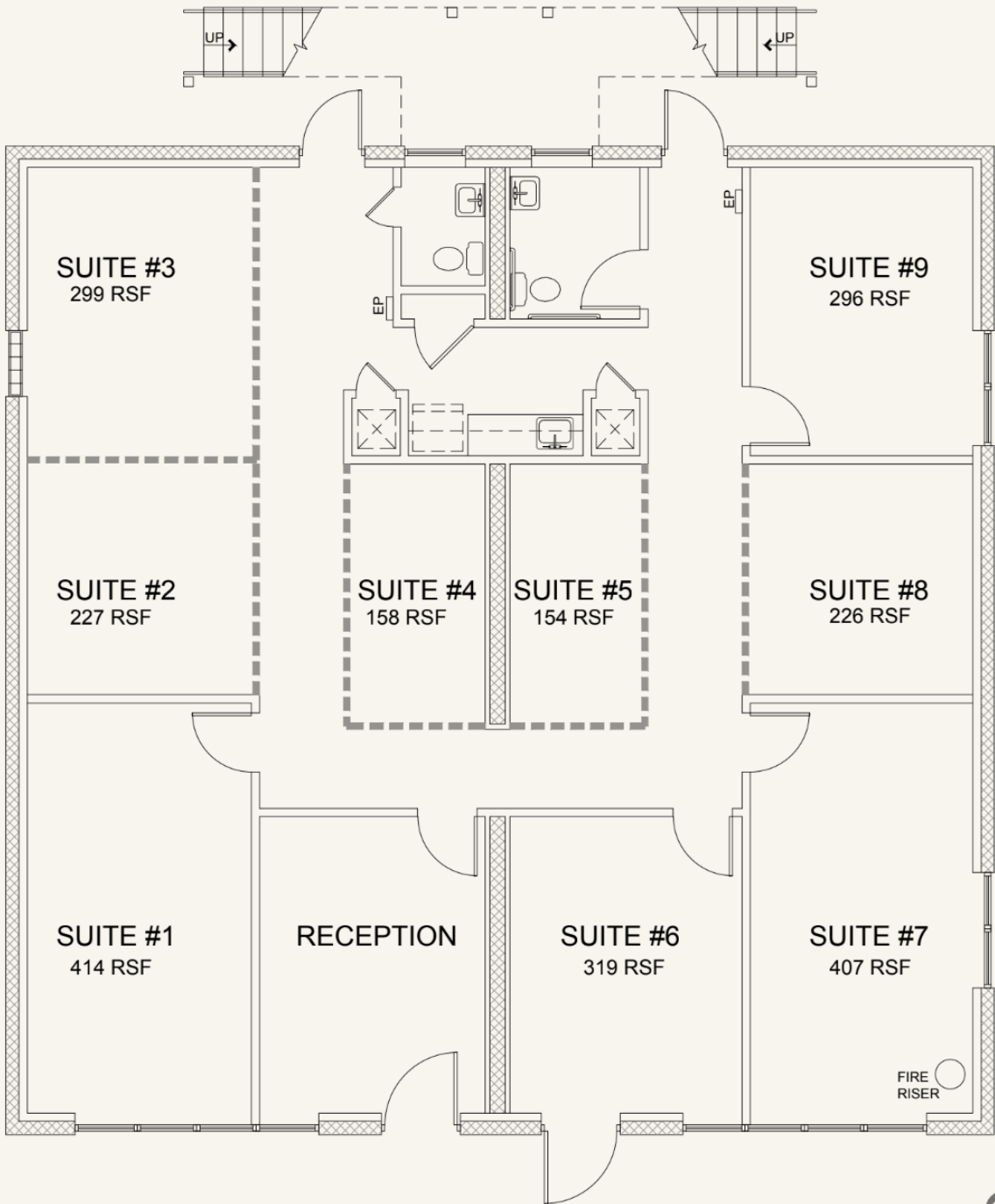
LEVEL 1 - OFFICE/RETAIL
