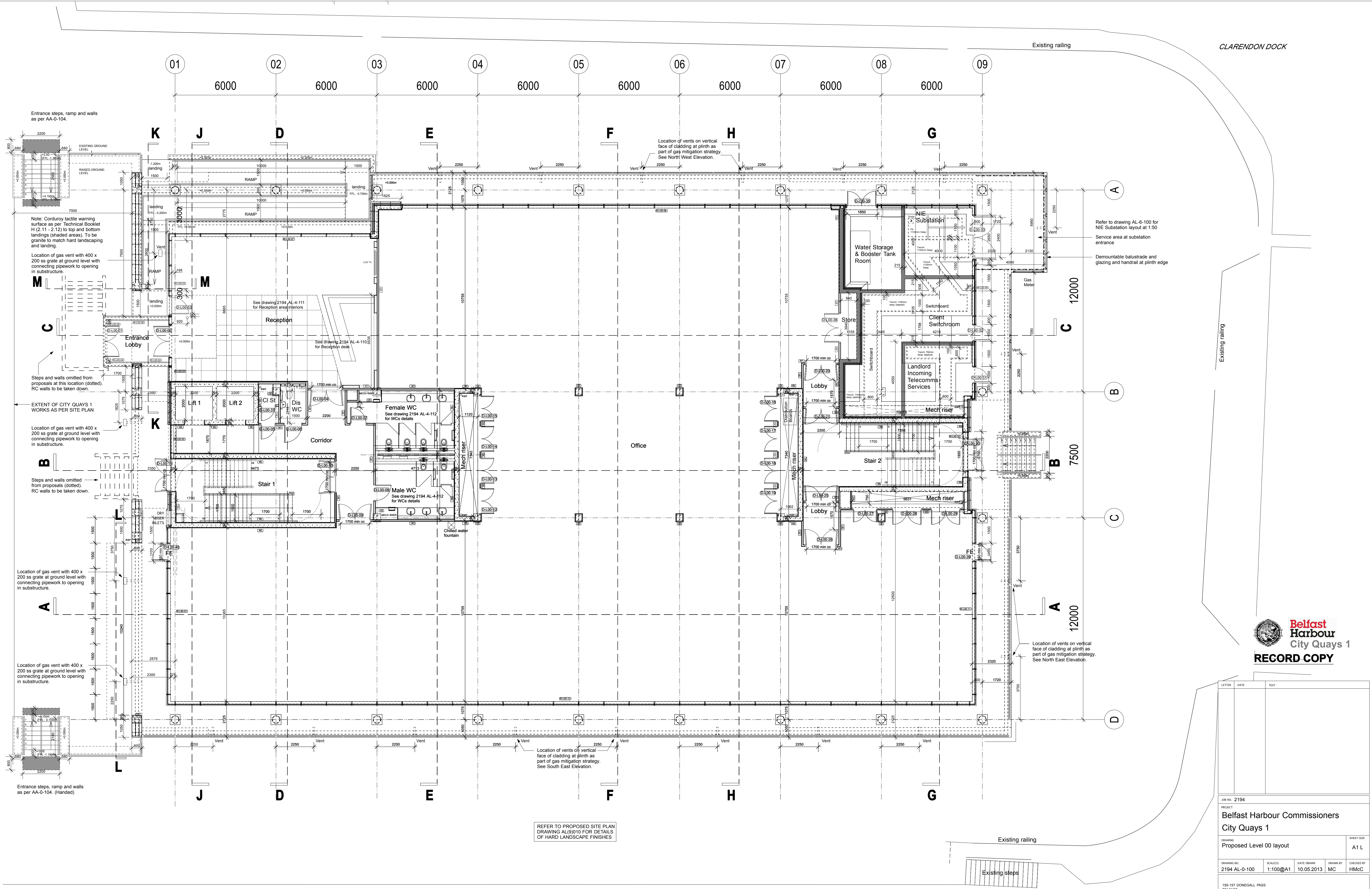
PROPOSED LEVEL 00 LAYOUT 1:100
