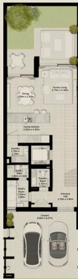
GROUND FLOOR
