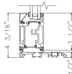
Low Sill
