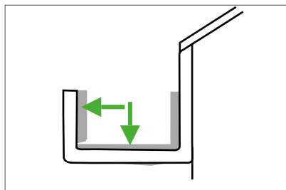
Gutter, edge and corner details
