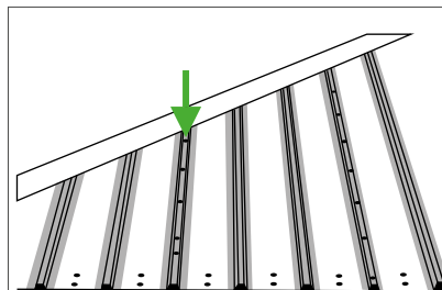
Joints between metal roof panels
