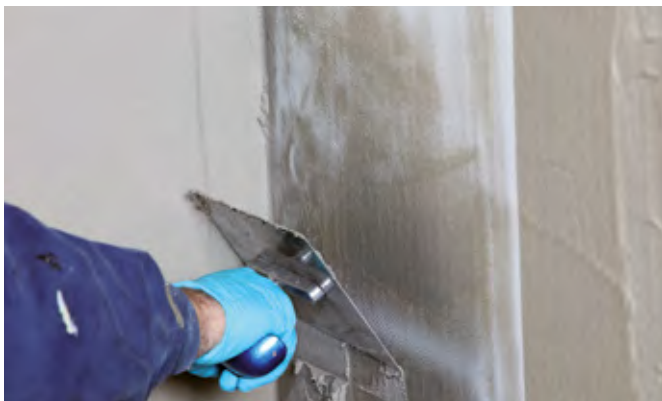
Application of the first layer of KÖSTER NB Elastic grey to the wall with brush or trowel. KÖSTER Flex Fabric is embedded into the fresh first layer.
