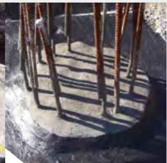
Connection of the area waterproofing (KÖSTER Deuxan 2C) to the pile head waterproofing.
