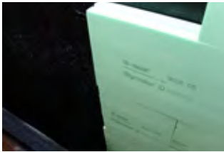
Insulation boards can be easily attached with two-component KÖSTER PMBCs. It is important the insulation boards are fully bonded.
