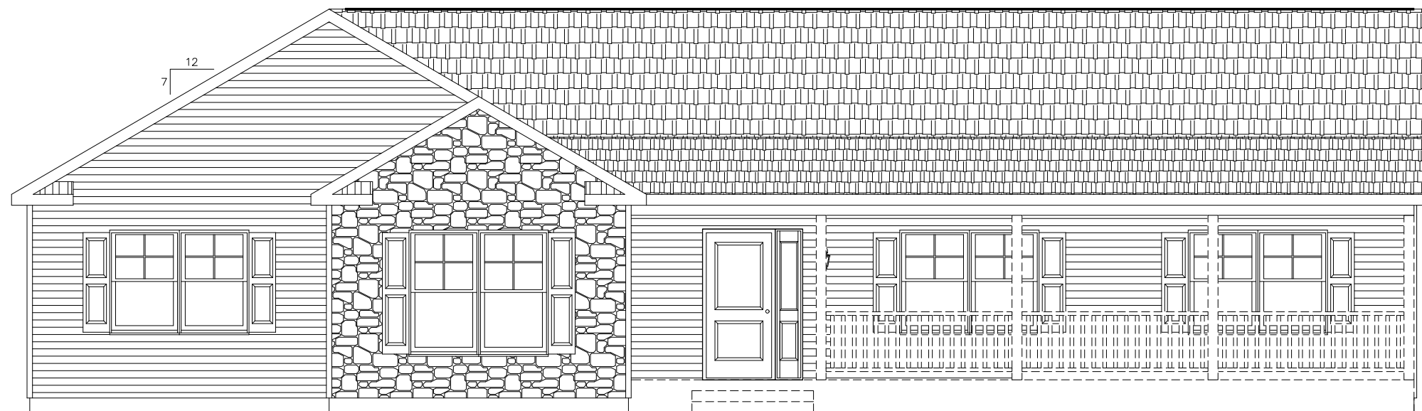
FRONT ELEVATION
