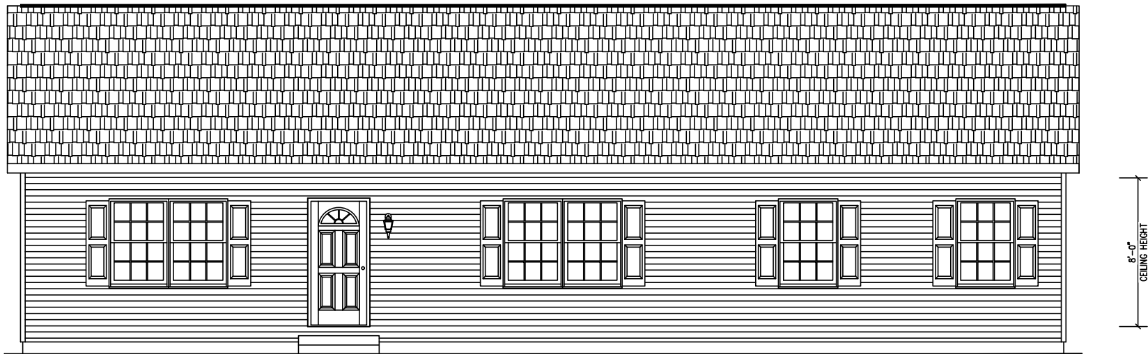
FRONT ELEVATION
