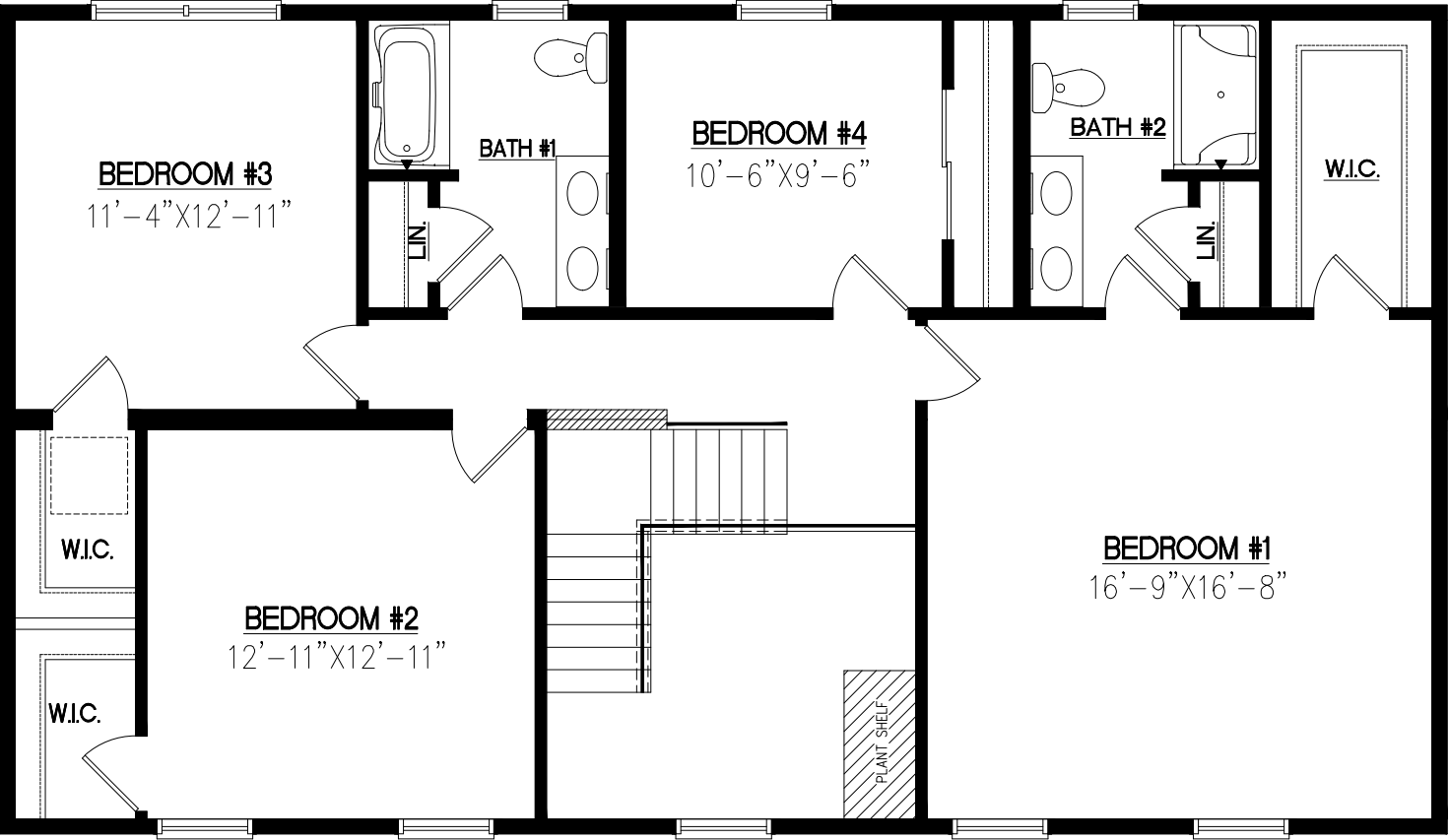
TWO STORY SECOND STORY FLOOR
