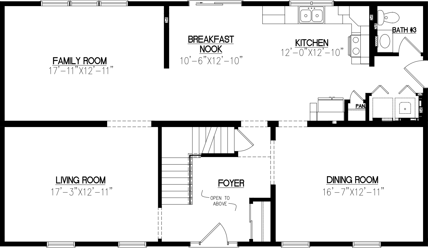
TWO STORY FIRST STORY FLOOR
