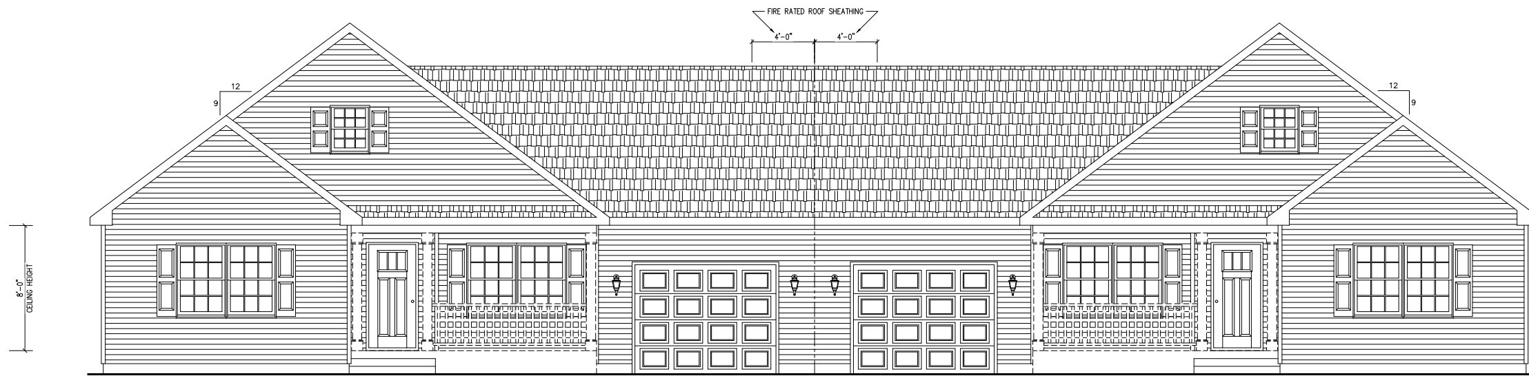
FRONT ELEVATION
