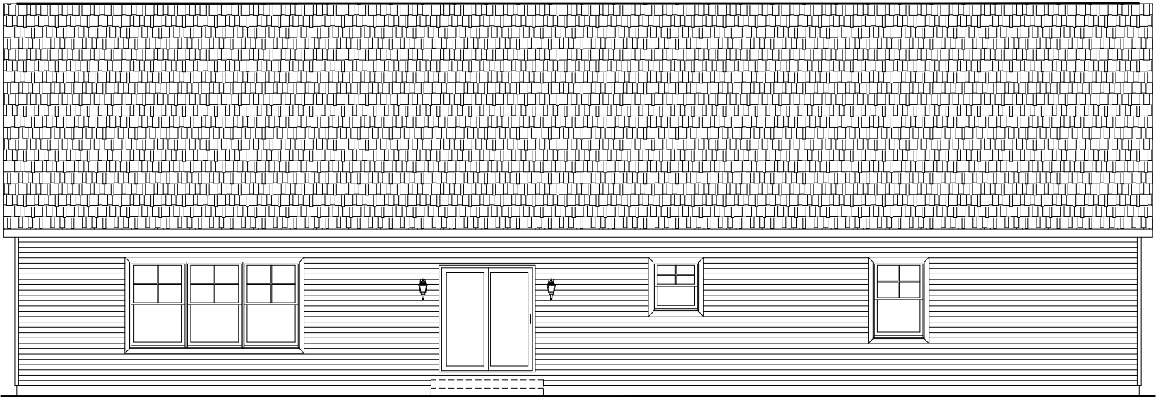
REAR ELEVATION
