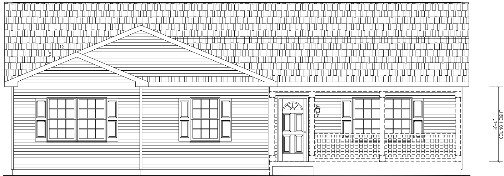
FRONT ELEVATION
