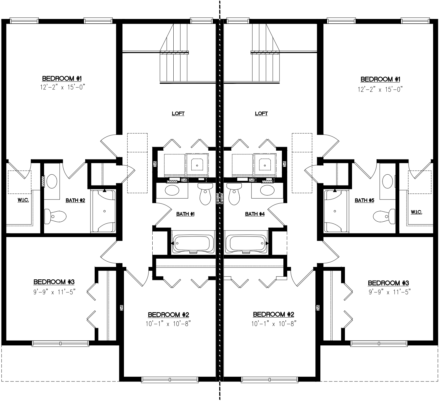
TWO STORY SECOND STORY FLOOR
