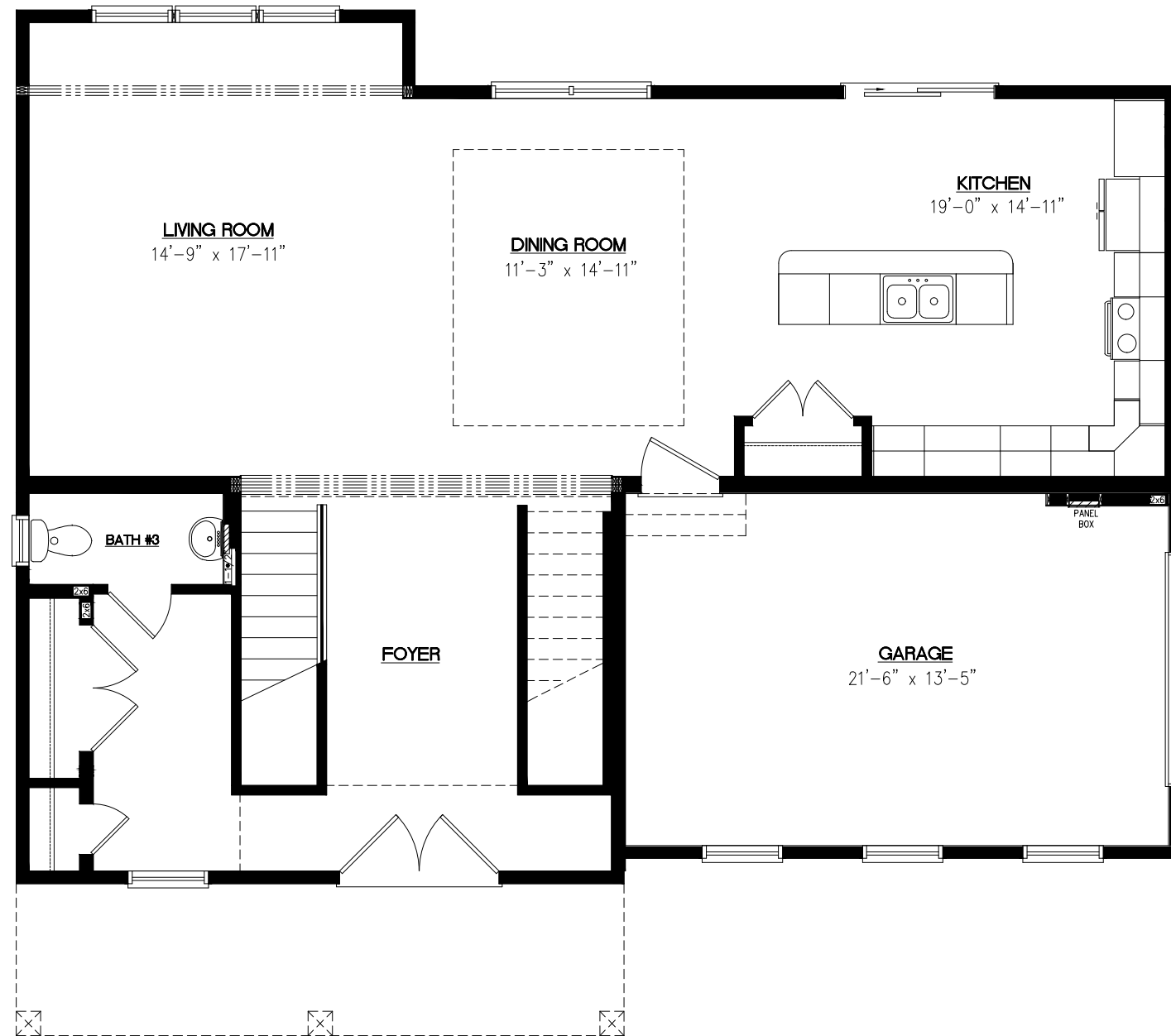
FIRST STORY FLOOR TWO STORY
