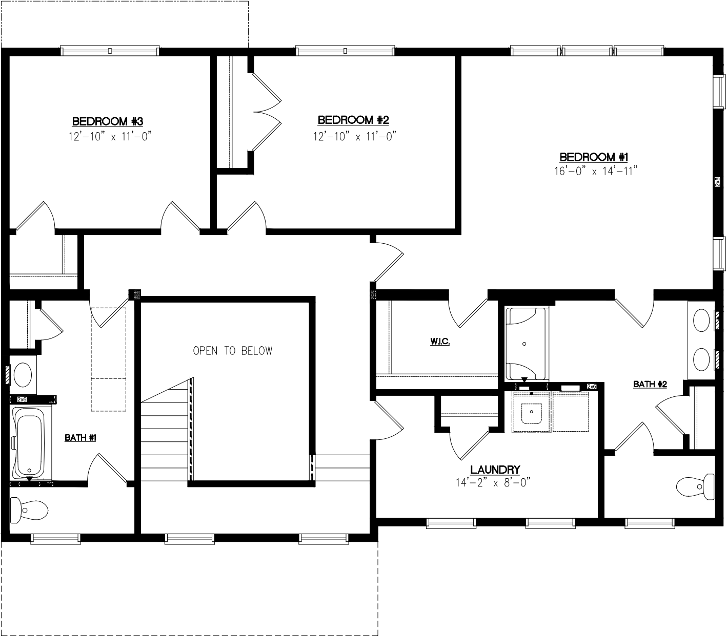
SECOND STORY FLOOR TWO STORY
