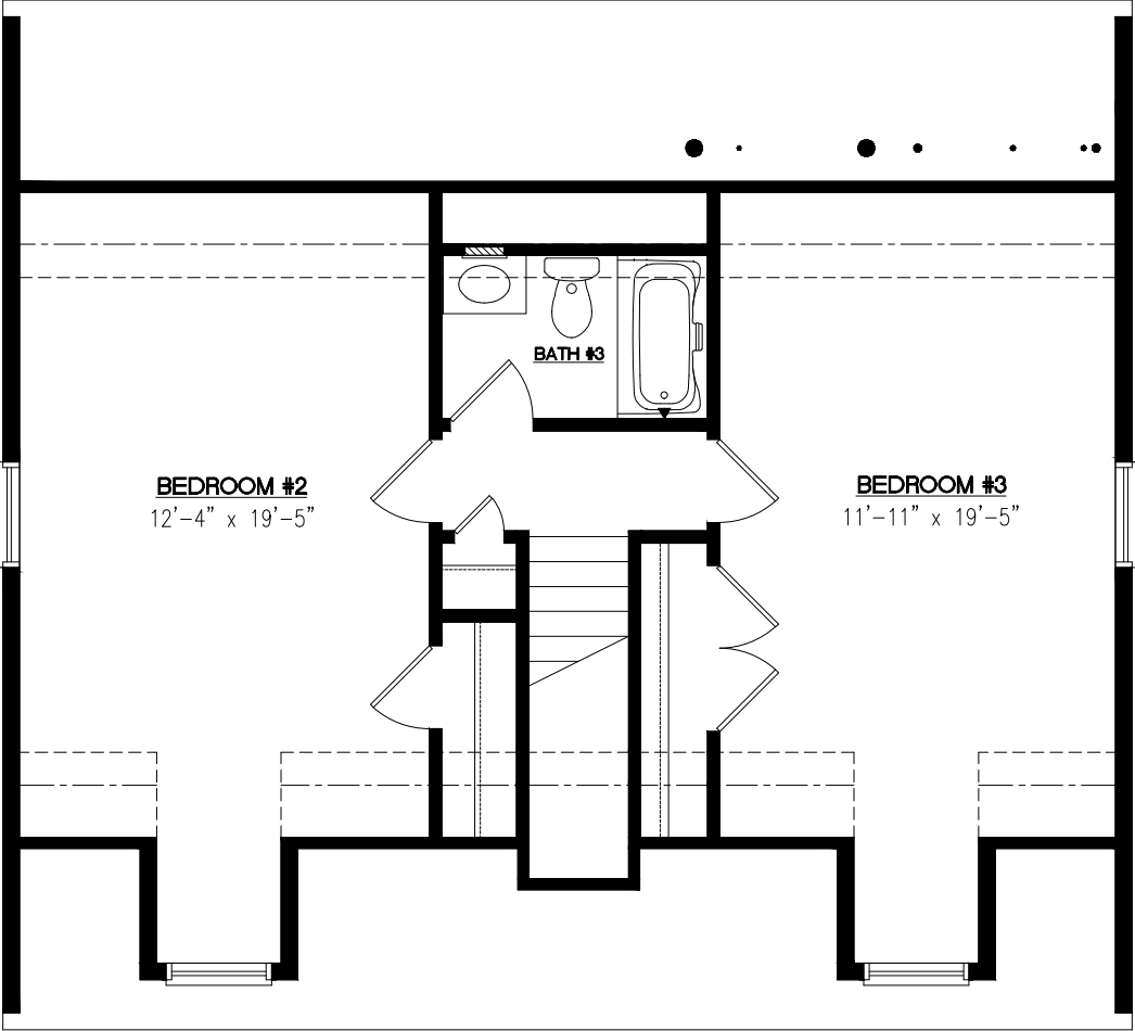
CAPE SECOND STORY FLOOR
