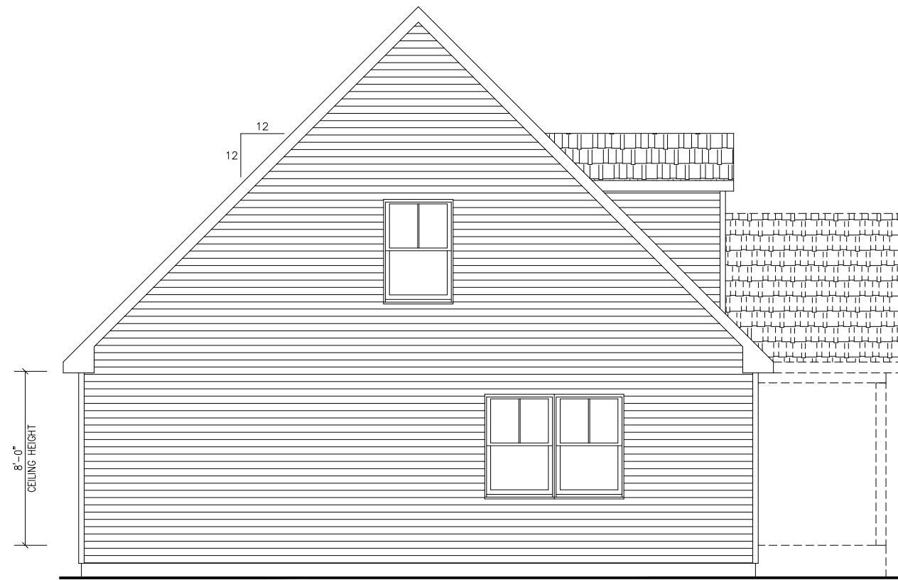
LEFT ELEVATION
