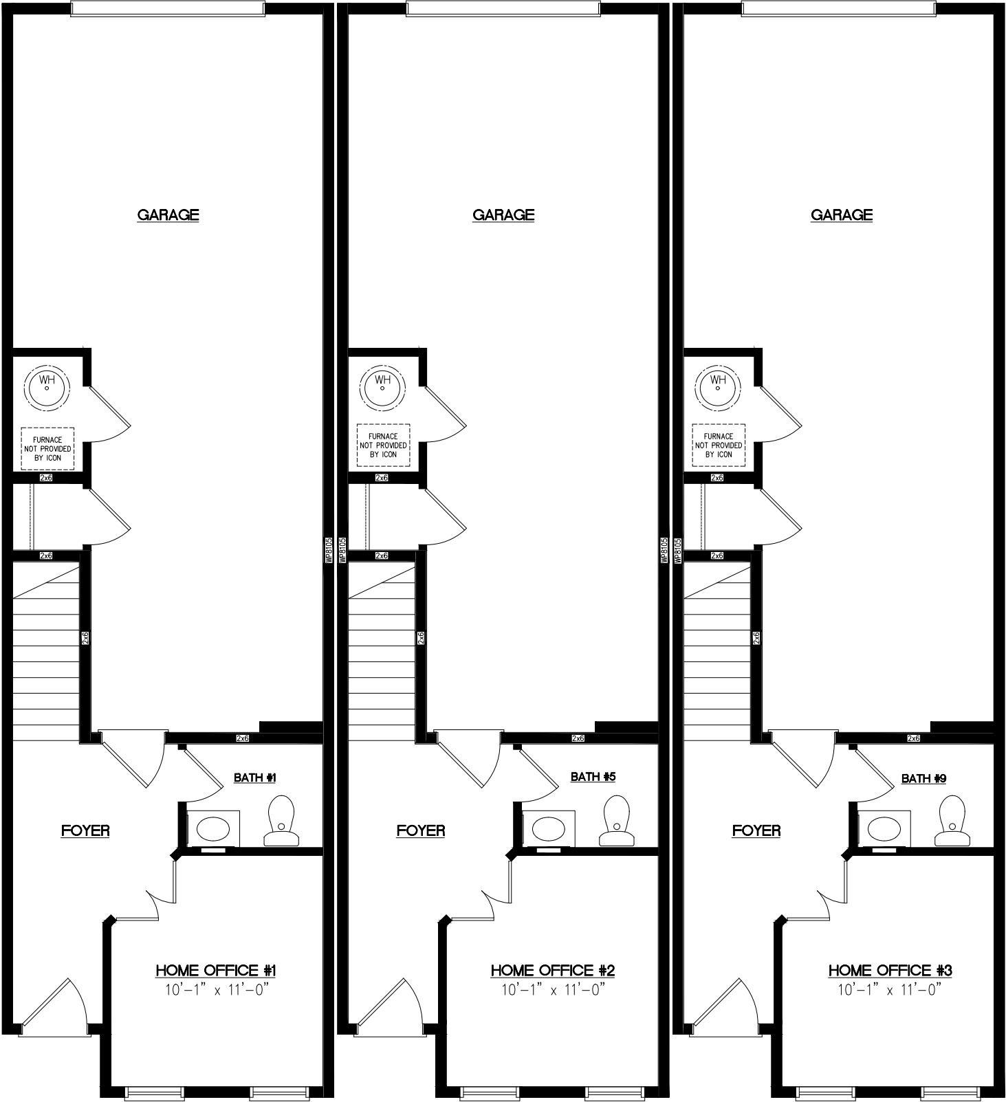
3-STORY TRIPLEX FIRST STORY FLOOR
