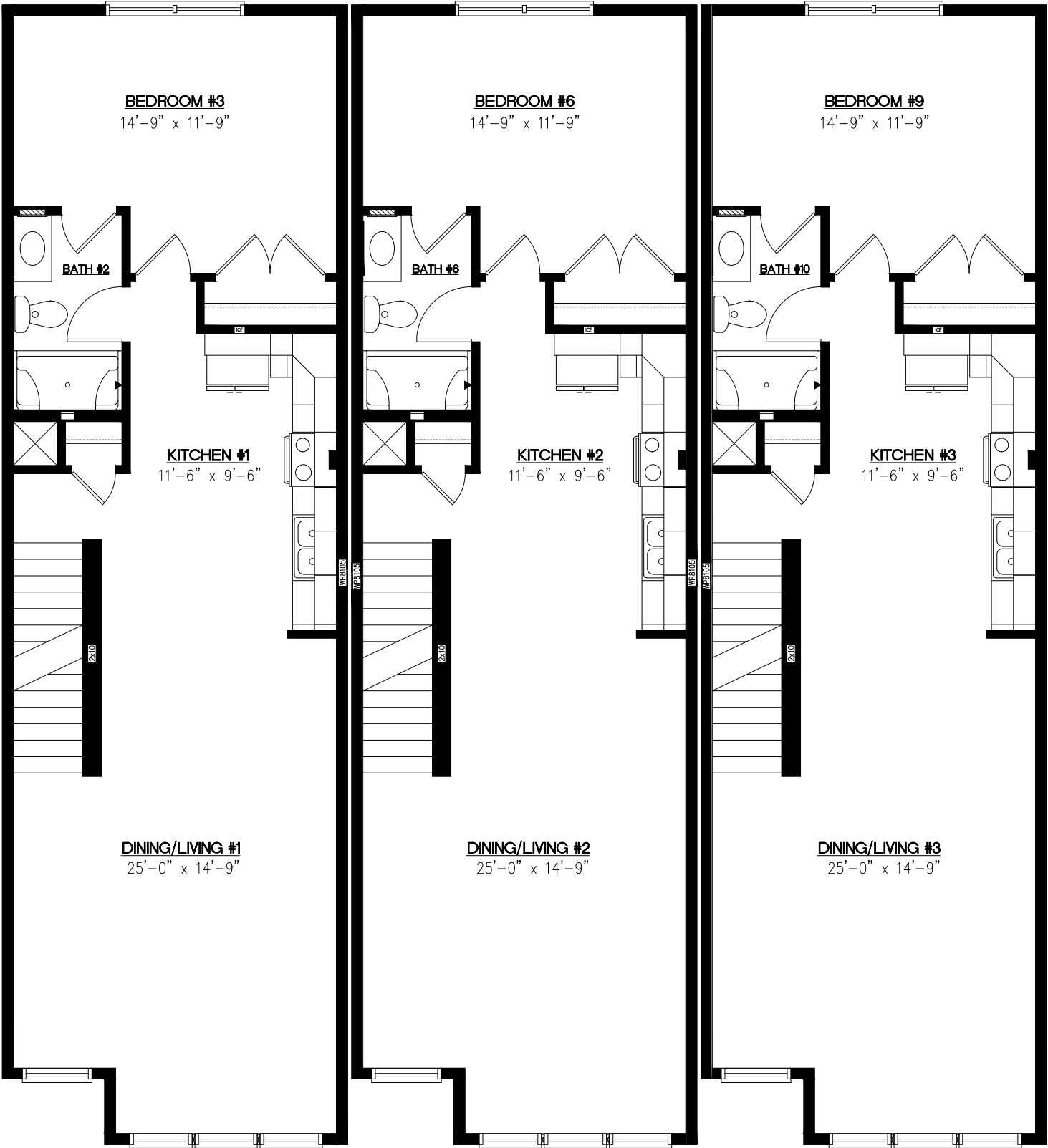
3-STORY TRIPLEX SECOND STORY FLOOR
