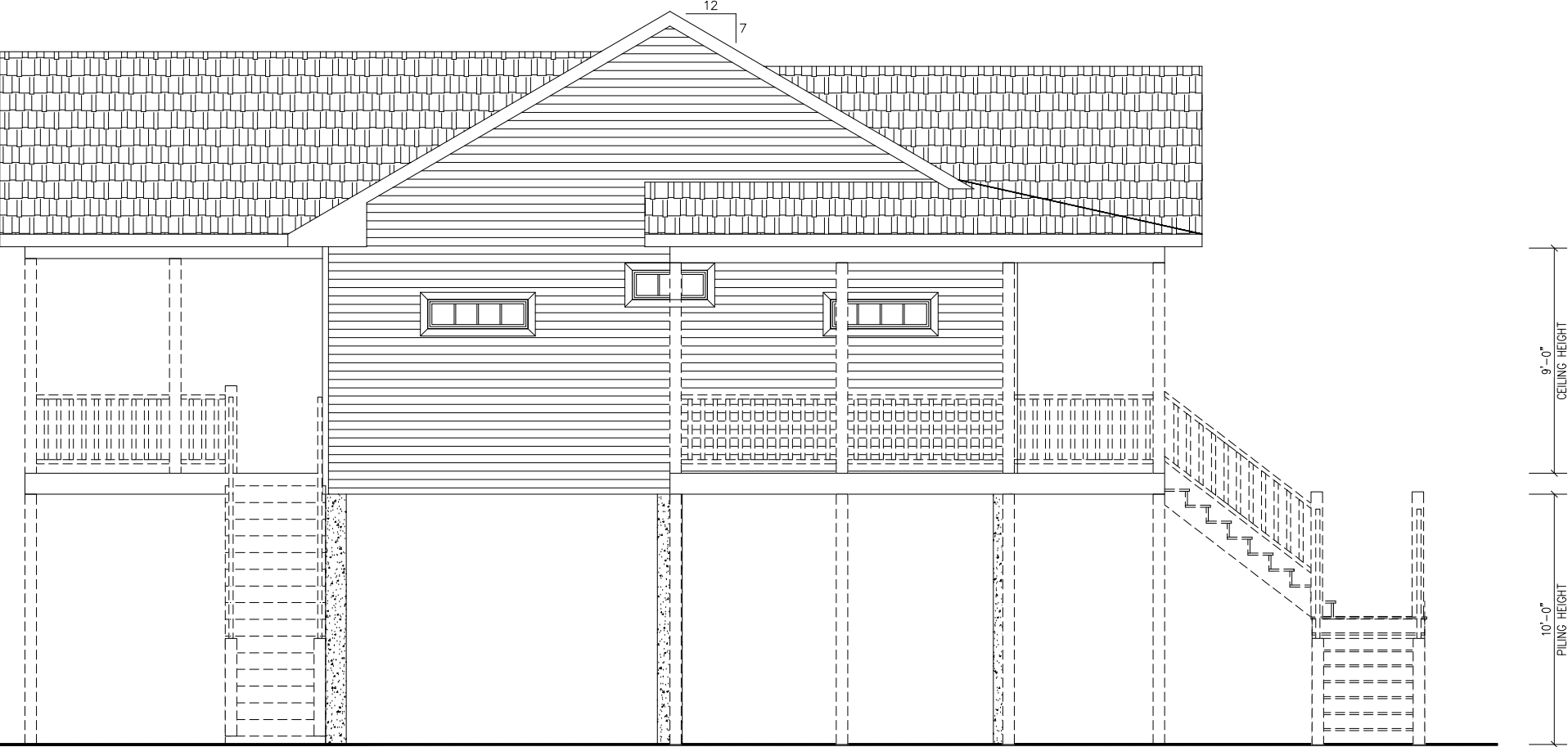
LEFT ELEVATION
