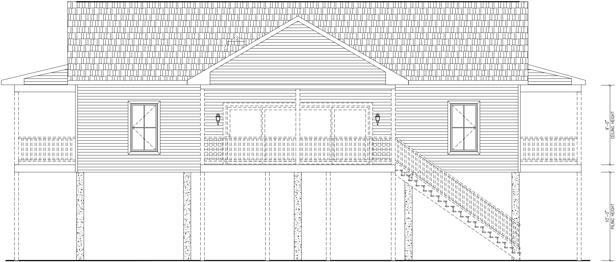
REAR ELEVATION
