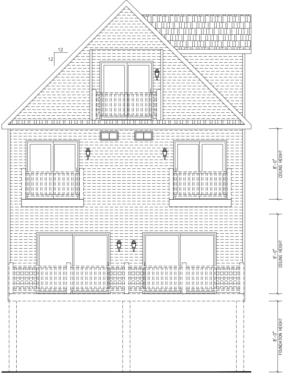
FRONT ELEVATION
