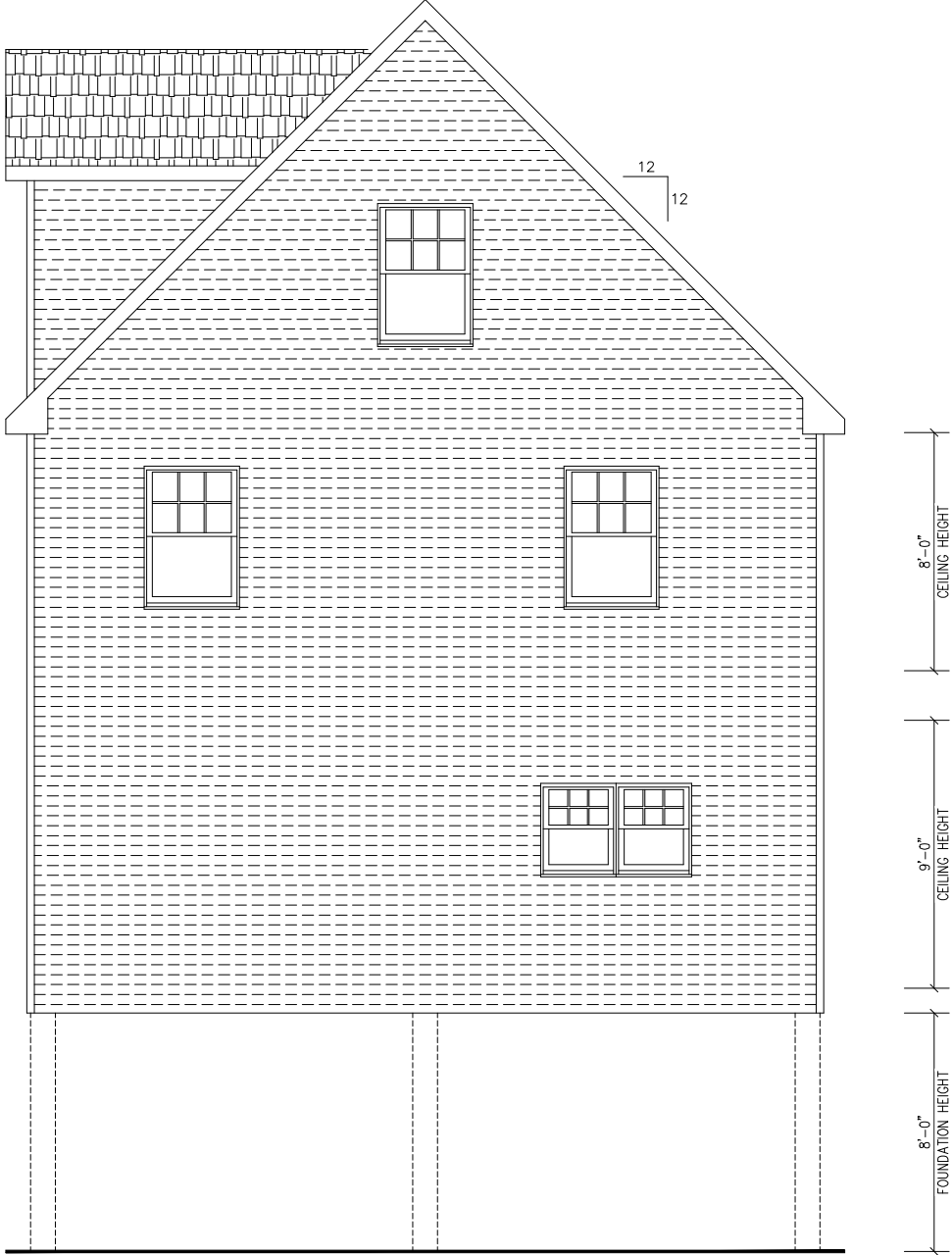
REAR ELEVATION
