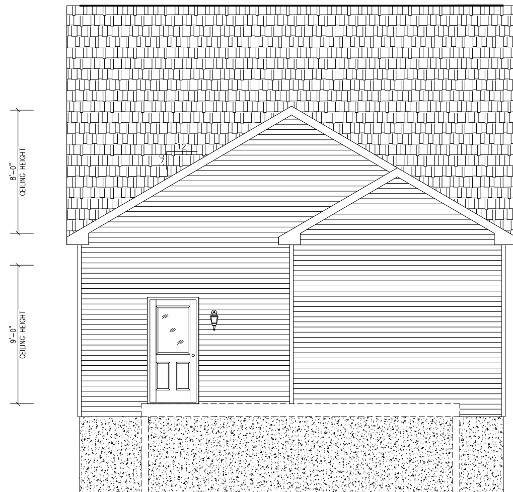
REAR ELEVATION
