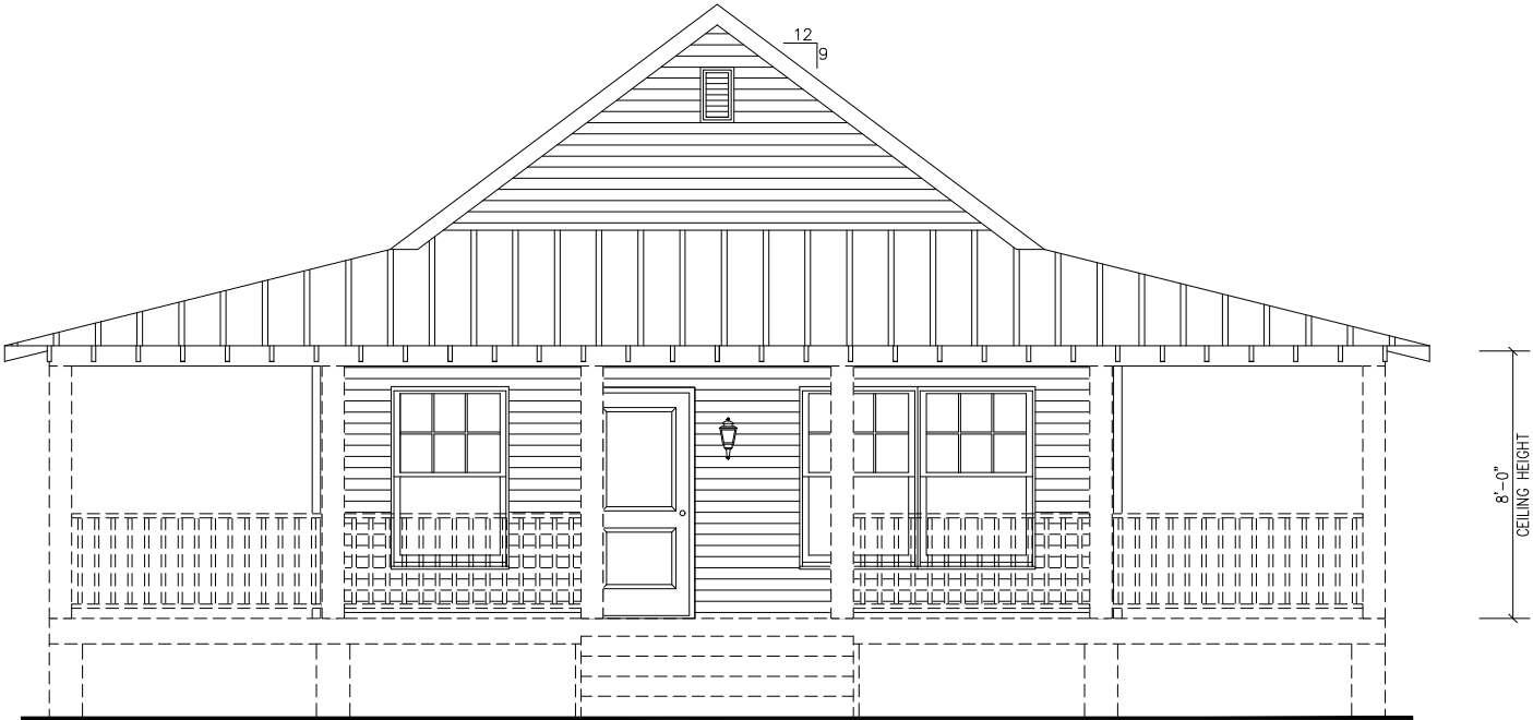
FRONT ELEVATION
