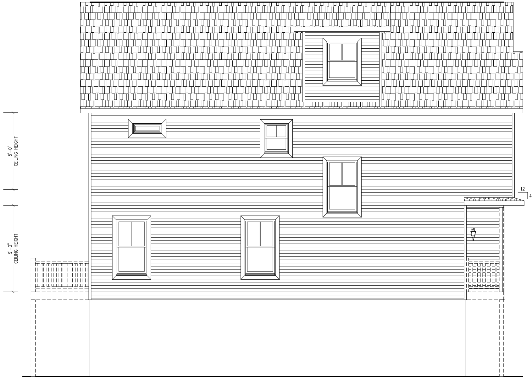
LEFT ELEVATION
