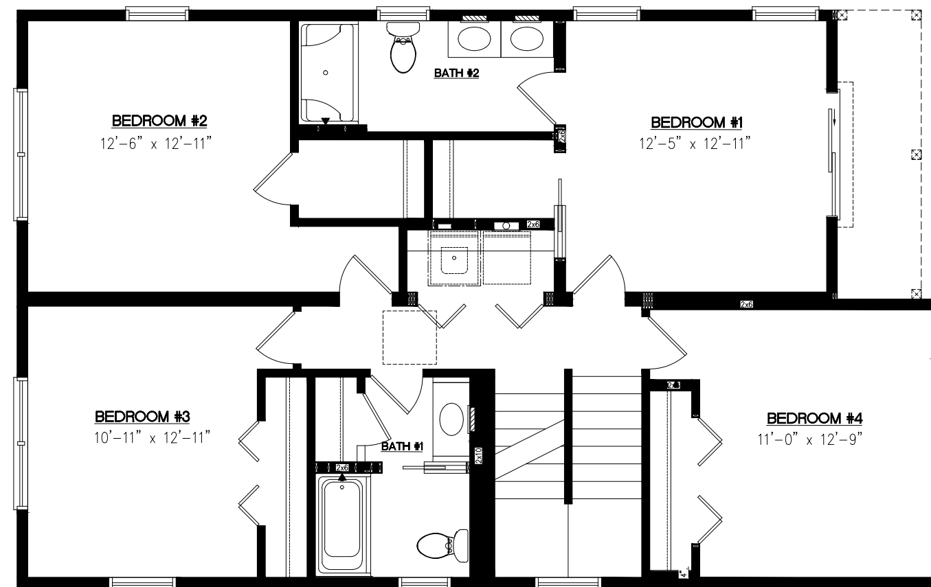
SECOND STORY FLOOR TWO STORY
