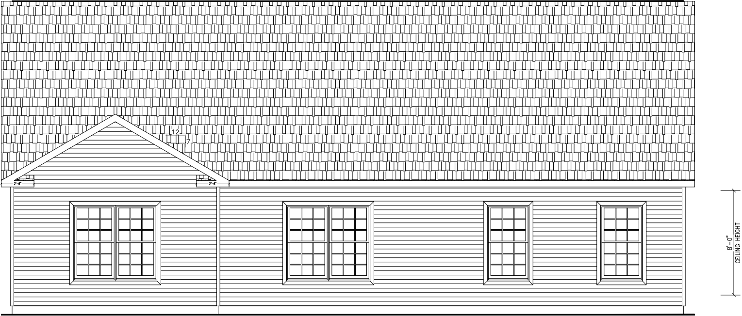
REAR ELEVATION
