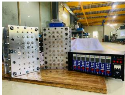
Blood collecting Tube Cap Mould
