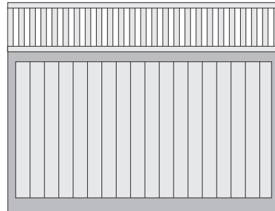
6 x 8' RC T & G Closed 1.5" Square Picket Topper
