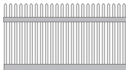
4 x 8' RC 1.5" Square Picket 1.75" Spaced Straight Pyramid Top
