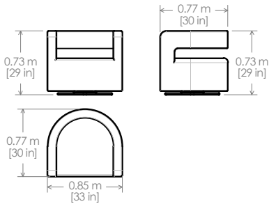
SW SWIVEL CHAIR SILLON GIRATORIO
