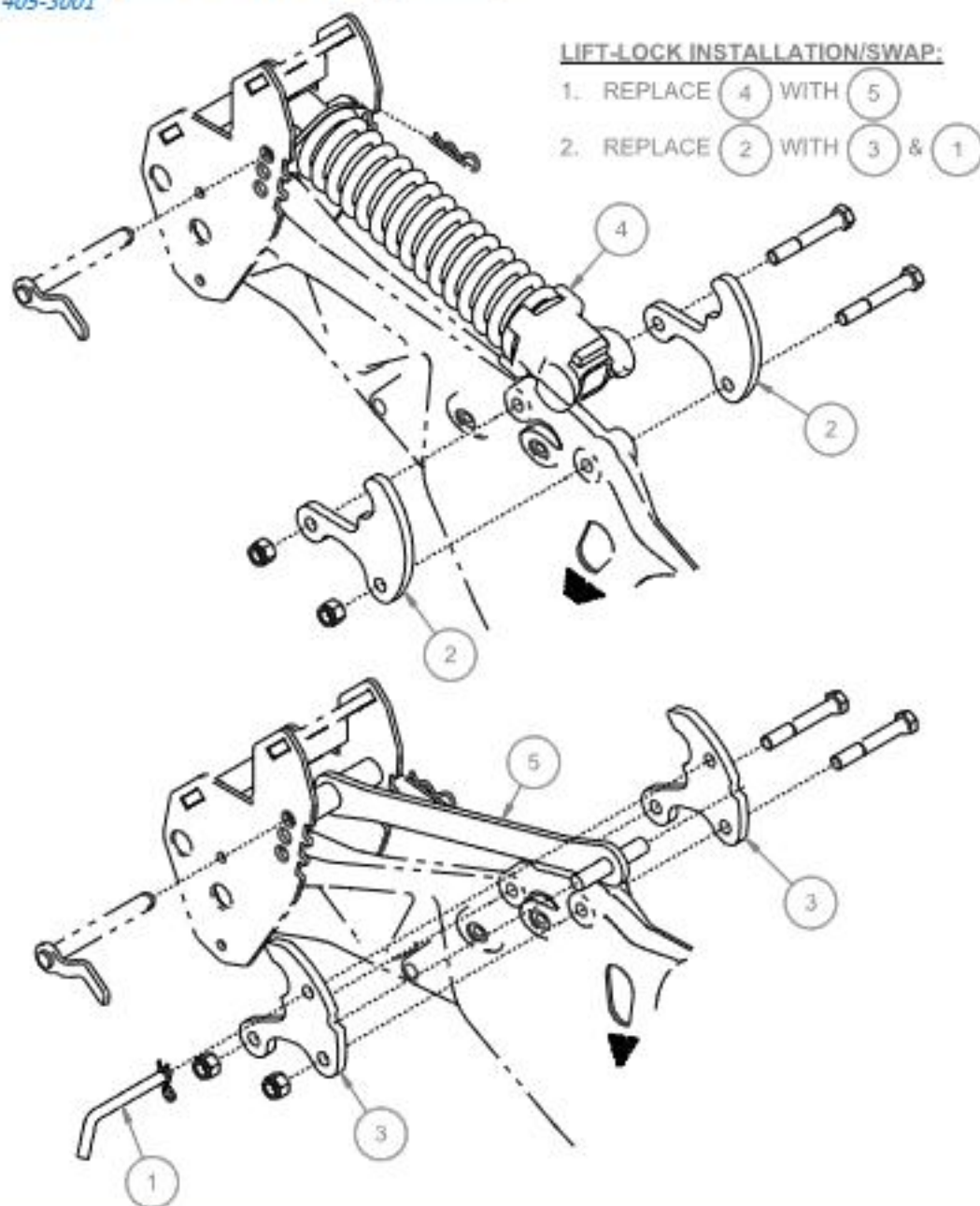
MK III Opener Lift-lock Kit
