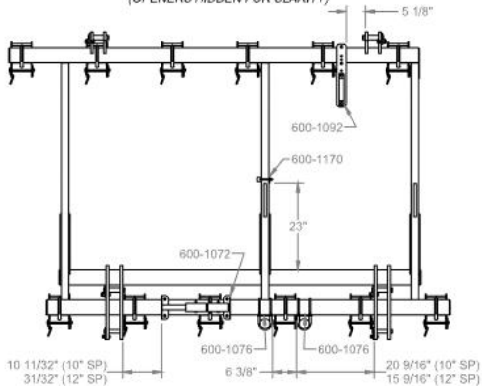
OUTER RH SUBFRAME (OPENERS HIDDEN FOR CLARITY)
