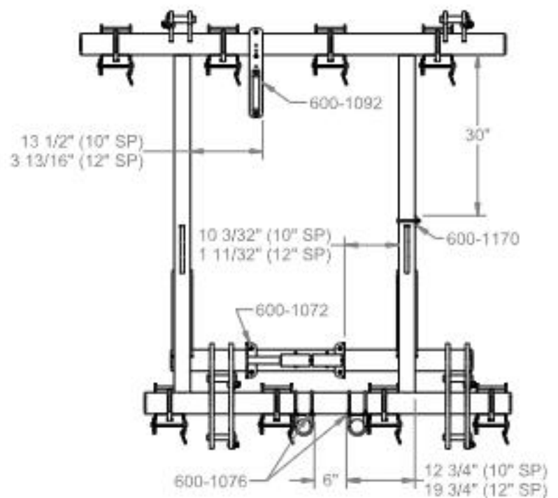
RH SUBFRAME (OPENERS HIDDEN FOR CLARITY)
