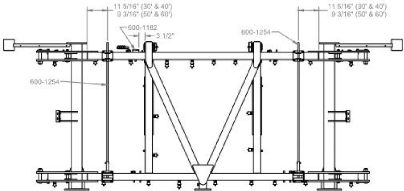
CENTER FRAME
