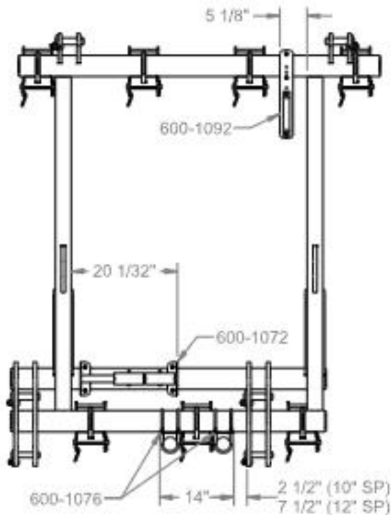
LH SUBFRAME (OPENERS HIDDEN FOR CLARITY)
