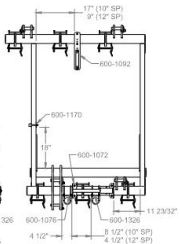
OUTER RH SUBFRAME (OPENERS HIDDEN FOR CLARITY)
