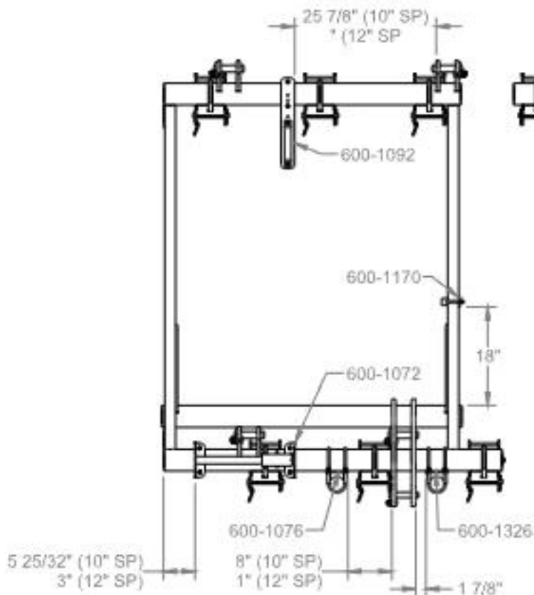
OUTER LH SUBFRAME (OPENERS HIDDEN FOR CLARITY)
