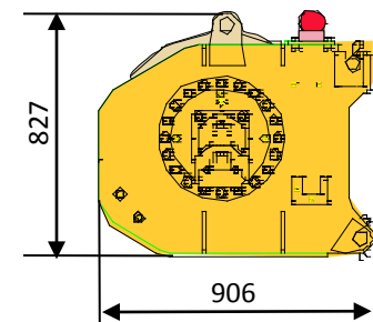
副起升机构 ( 含钢丝绳 ) 1920kg Auxiliary winch ( rope included )
