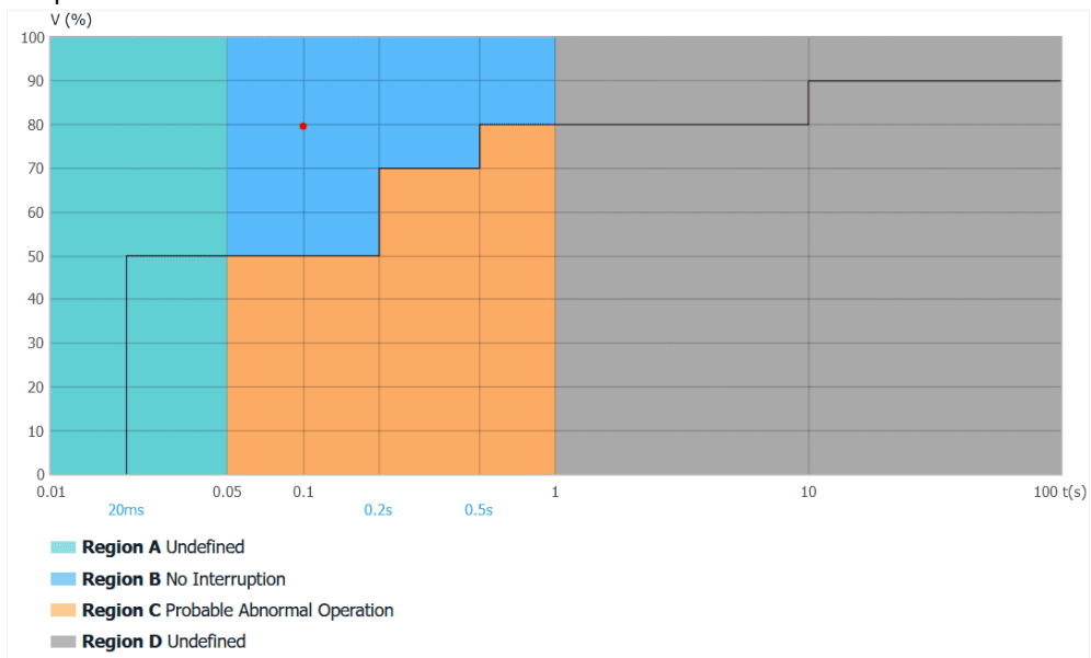
Figure 4-20 SEMI F47 Plot Descriptions
