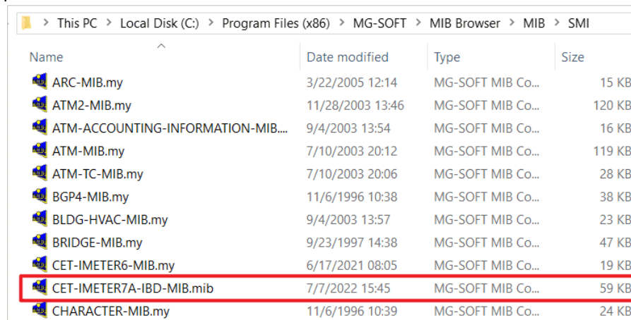
Figure 4-45 Save the MIB Definition File to SMI Folder
