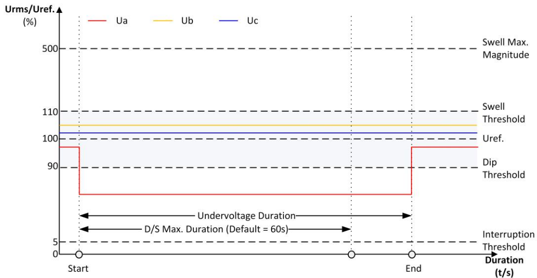
Figure 4-9 Undervoltage Detection Criteria
