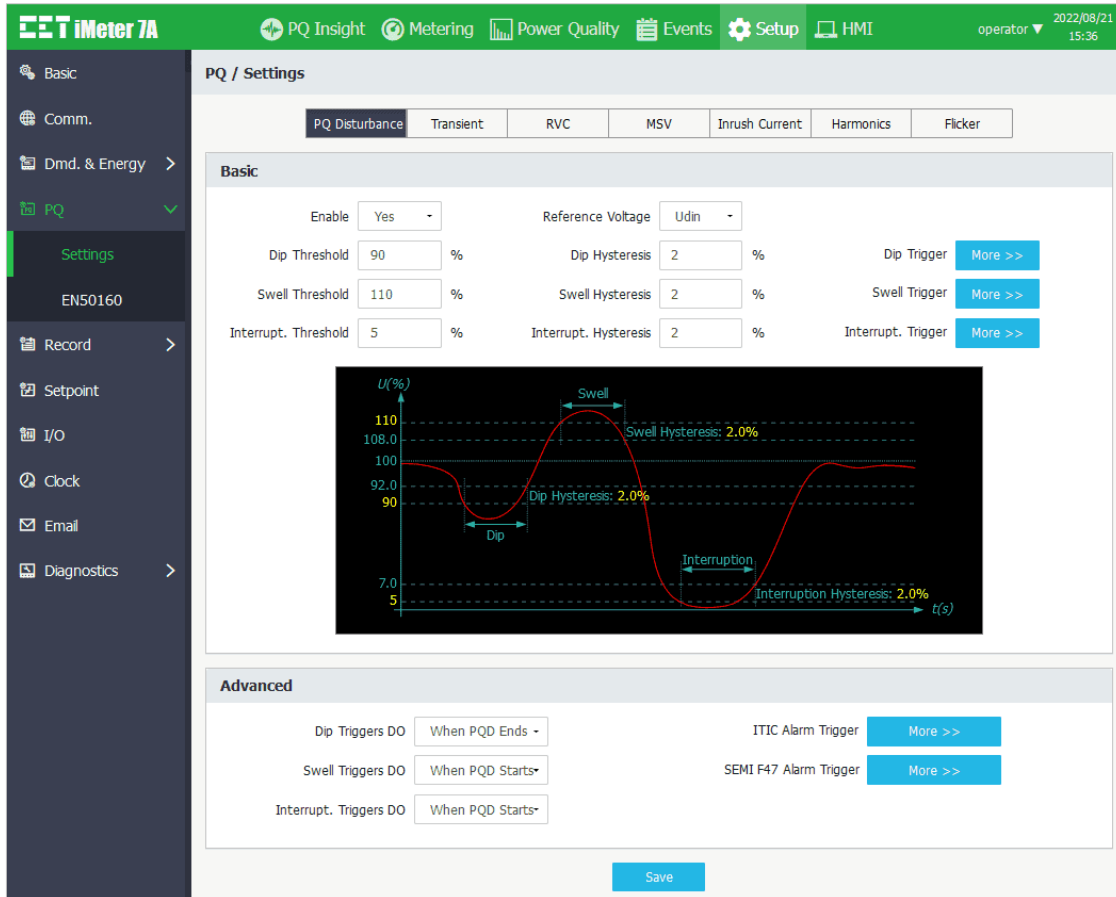
Figure 3-126 PQ Disturbance Settings Interface
