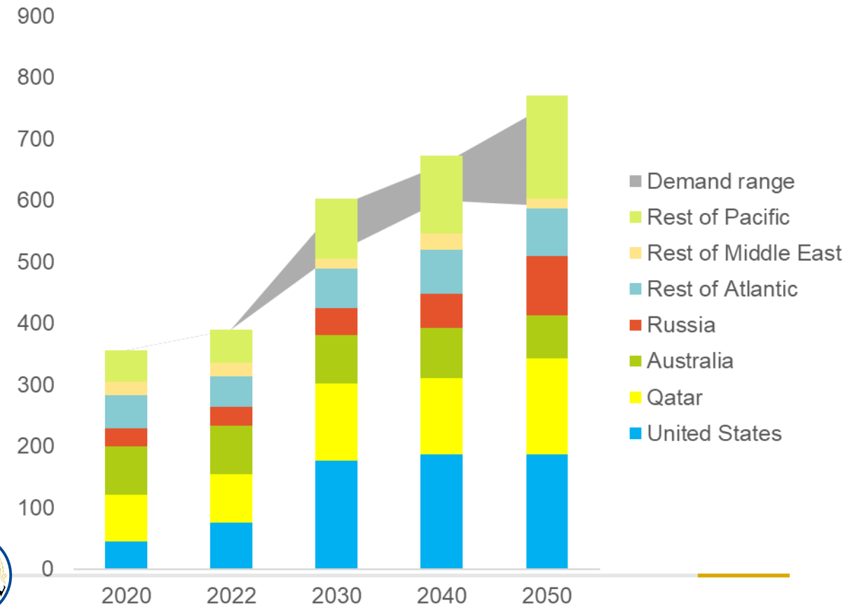
Long Term Supply and Demand for LNG (Mt)
