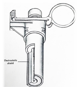
FIGURE 6-C Cutaway drawing showing shielding imbedded near outer surface of fuse tube
