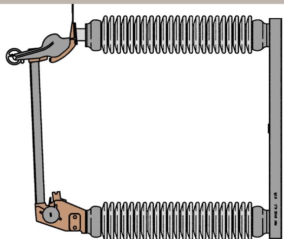
FIGURE 3 HPA 69 kV 200 AMP
