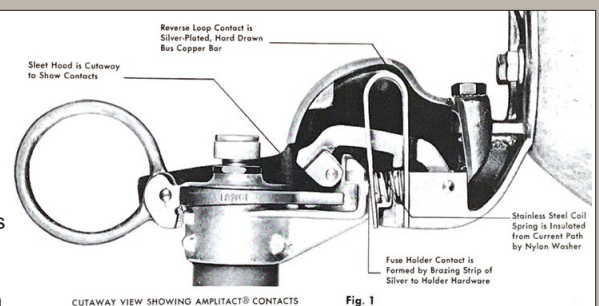
CUTAWAY VIEW SHOWING AMPLITACT® CONTACTS
