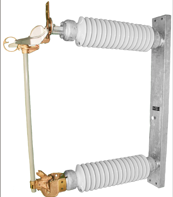
FIGURE 10 Fuse illustrated is a BPA 69 kV, 100 amp.
