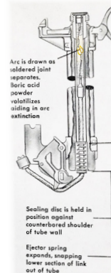
FIGURE 4-A Initial Stage of Low Fault
