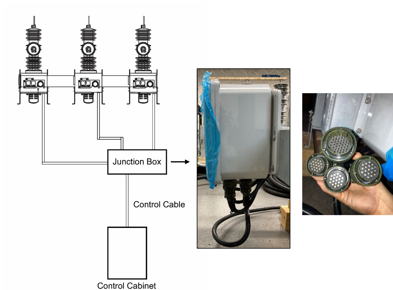
Figure 14: Typical Control System (Triple Tank Units)
