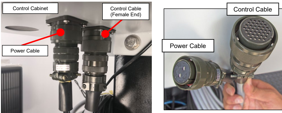
Figure 19: Power & Control Cable Connections
