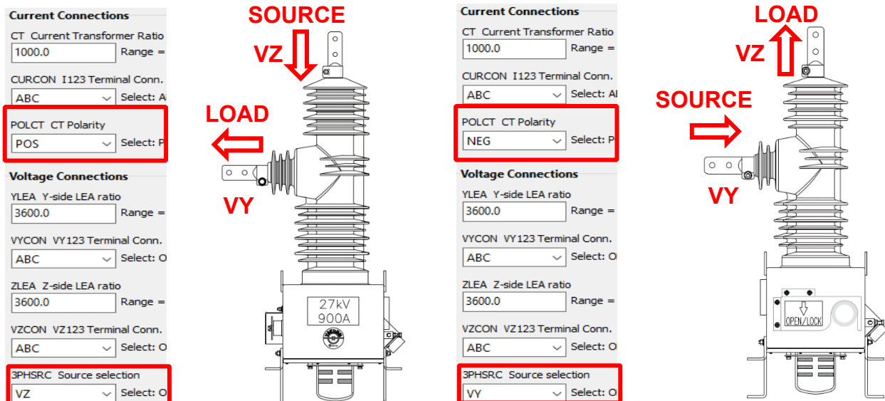
Figure 3: Recloser Source & Load Configuration
