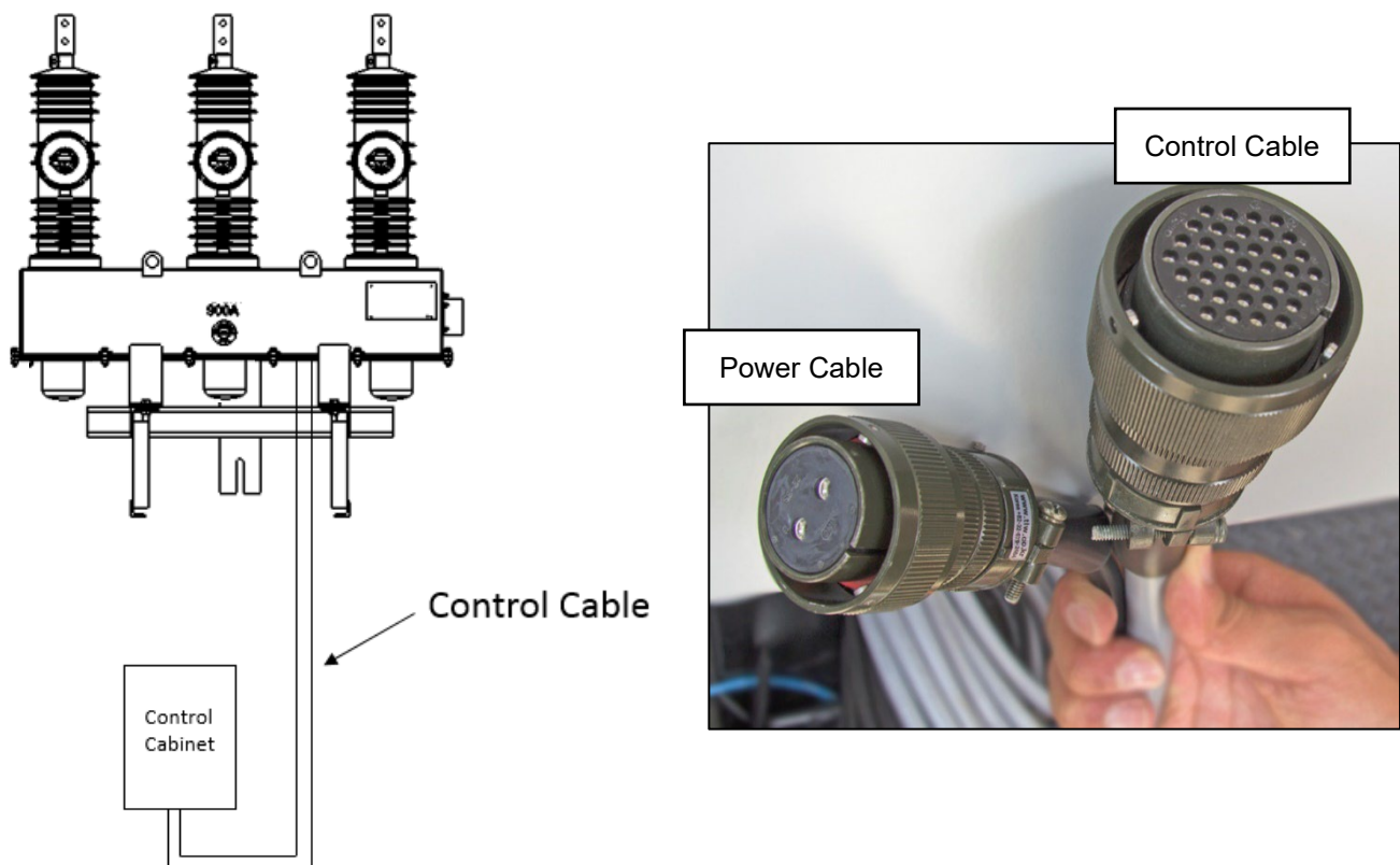
Figure 13: Typical Control System (Single Tank Units)
