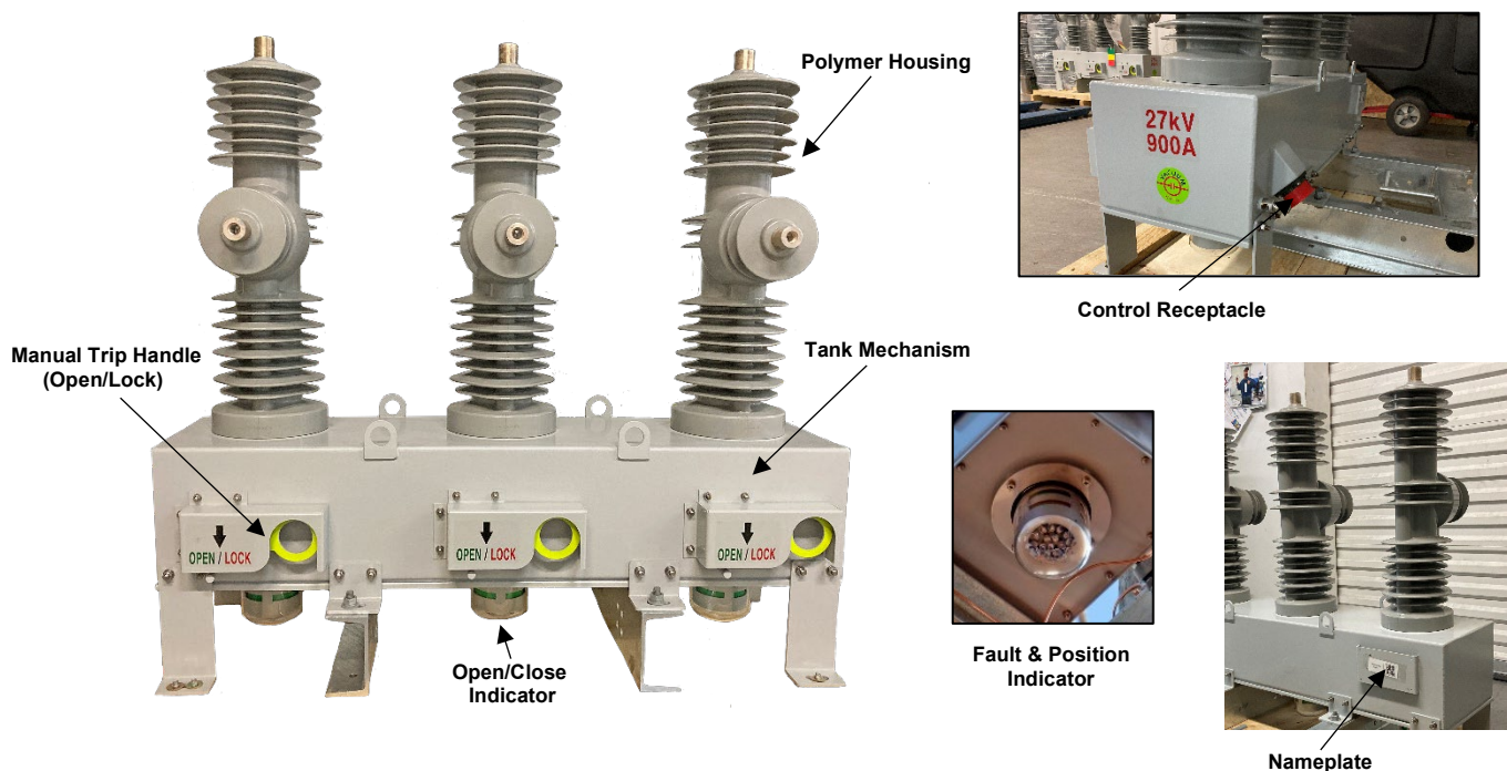
Figure 1: Typical Recloser Construction
