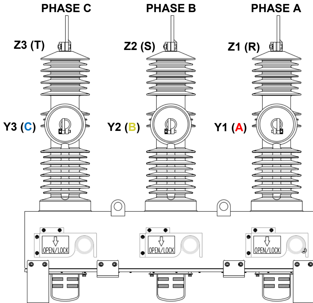
Figure 2: Recloser VY123 & VZ123 Voltage Terminal Connection Configuration
