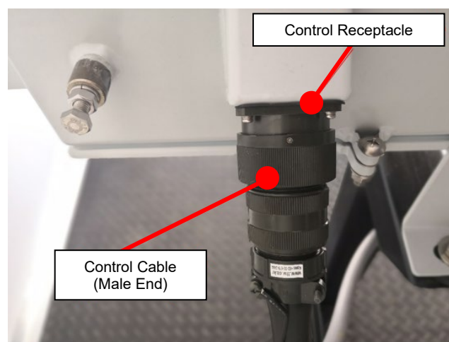
Figure 20: Control Cable Connection
