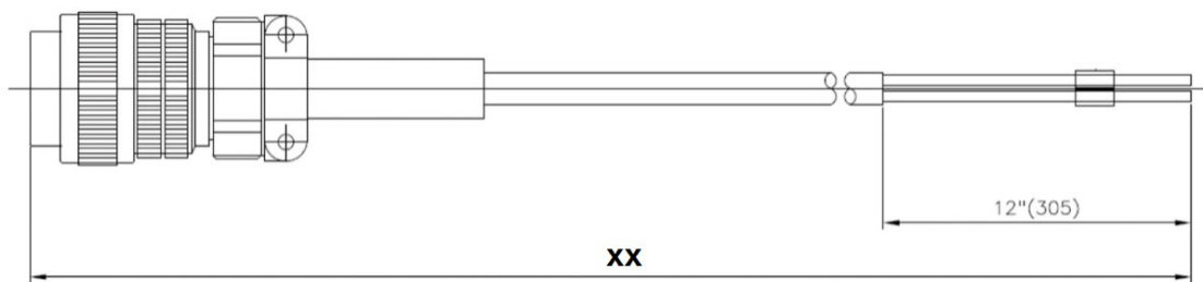
Figure 11: Power Cable
