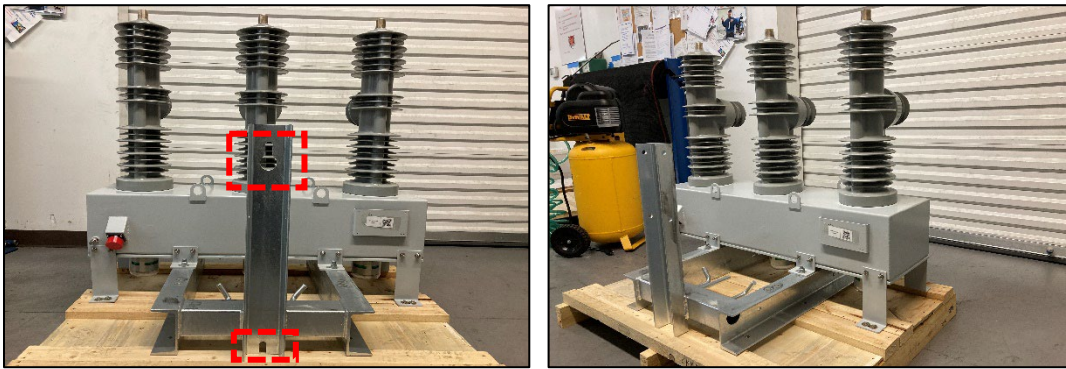
Figure 17: Single Tank Mounting
