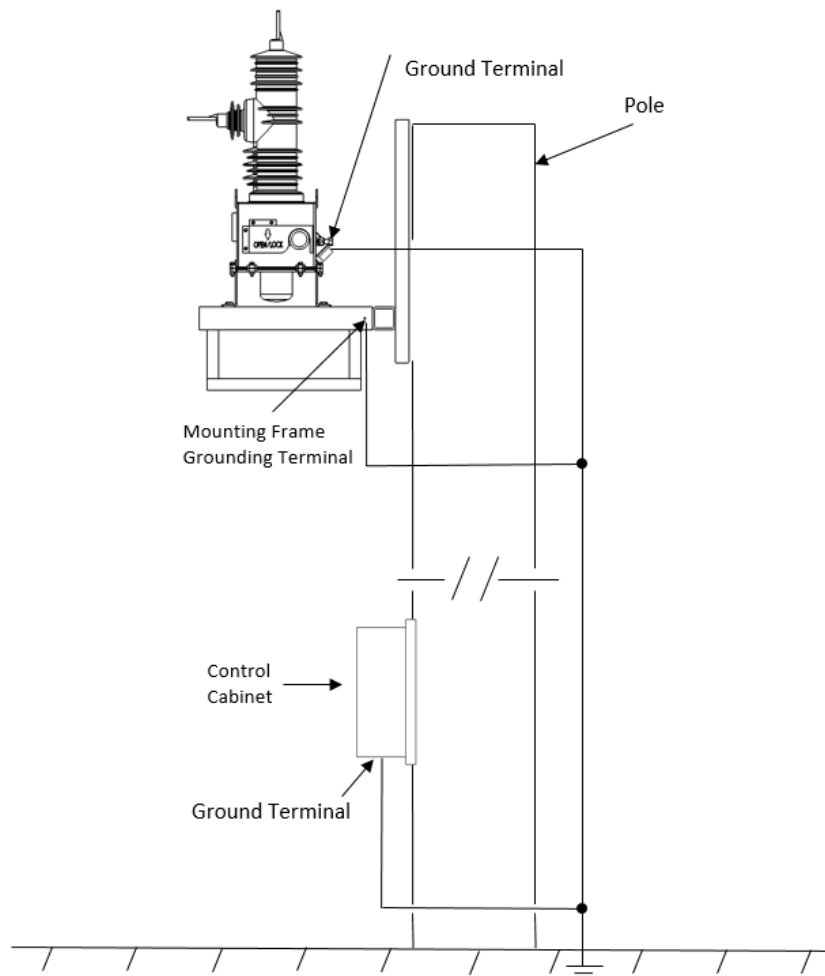
Figure 21: Recommended Grounding Method
