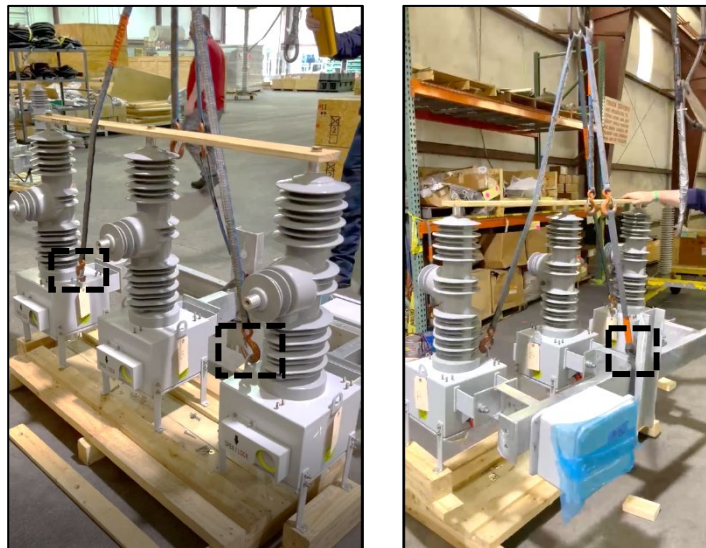
Figure 6: Tripod Lifting Arrangement (Triple Tank Units)
