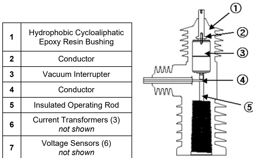
Figure 4: Interrupter Detail
