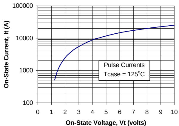
ON-STATE CURRENT CHARACTERISTIC
