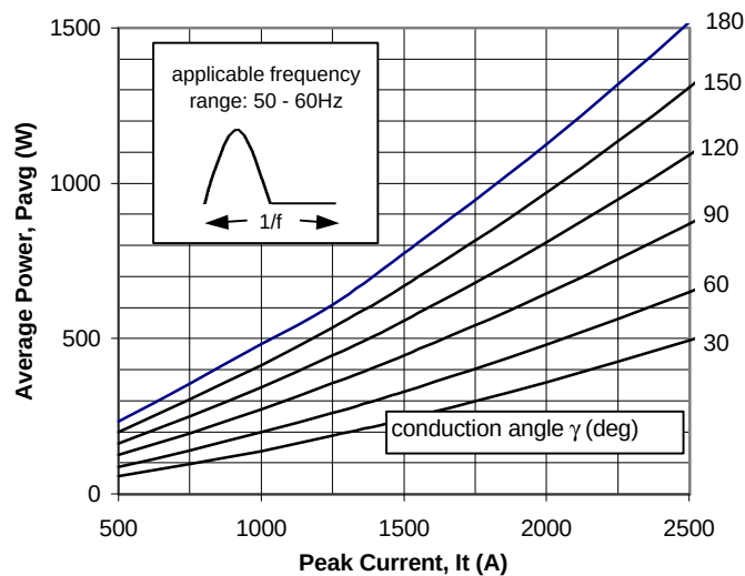
MAXIMUM FULL CYCLE AVERAGE POWER DISSIPATION SINE WAVE CURRENT FOR VARIOUS CONDUCTING ANGLES
