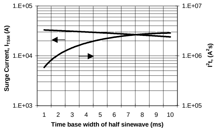
NON-REPETITIVE I_{TSM} AND I^2t CAPABILITY FOR FUSE COORDINATION
